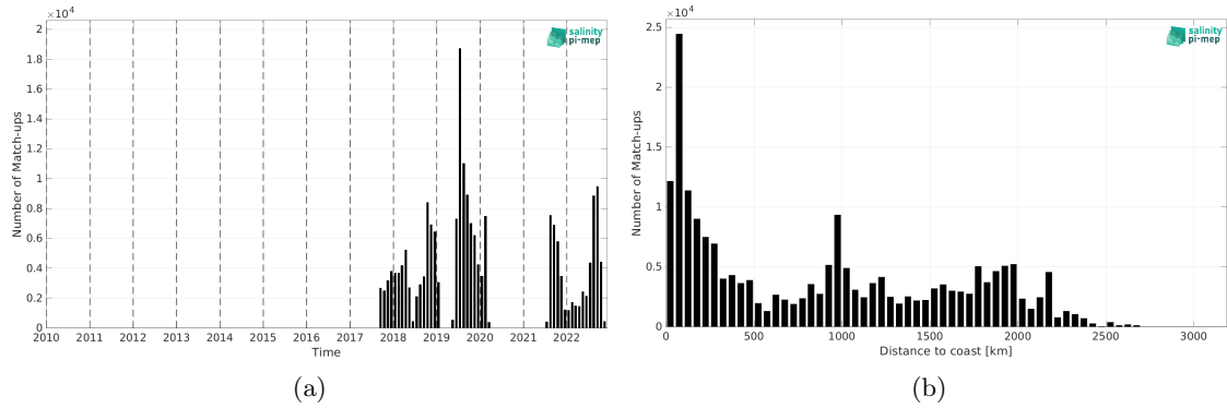
Figure 2: Number of match-ups between Saildrone and SMOS SSS L2 v700 (ESA) SSS as a function of time (a) and as function of the distance to coast (b) over the Mid-Low Latitudes 45N-45S Pi-MEP region and for the full satellite product period.
