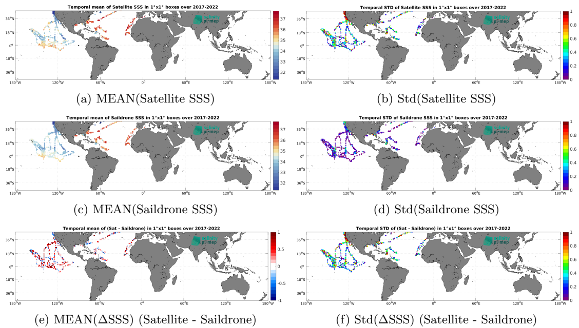
Figure 7: Temporal mean (left) and Std (right) of SSS from SMOS SSS L2 v700 (ESA) (top), Saildrone (middle), and of \Delta SSS (Satellite - Saildrone). Only match-up pairs are used to generate these maps.
