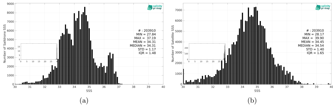
Figure 3: Histograms of SSS from Saildrone (a) and SMOS SSS L2 v700 (ESA) (b) considering all match-up pairs per bins of 0.1 over the Mid-Low Latitudes 45N-45S Pi-MEP region and for the full satellite product period.
