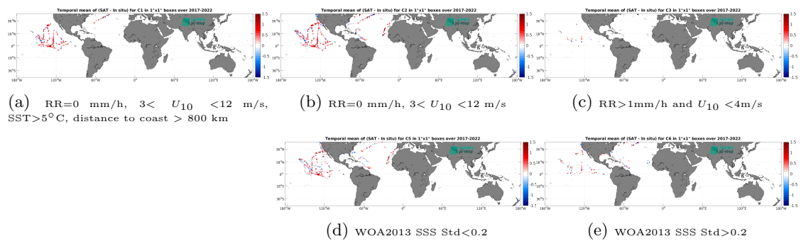
Figure 14: Temporal mean gridded over spatial boxes of size 1^\circ \times 1^\circ of \Delta SSS (SMOS SSS L2 v700 (ESA) - Sairdrone) for 5 different subdatasets corresponding to: RR=0 mm/h, 3 < U_{10} < 12 m/s, SST > 5°C, distance to coast > 800 km (a), RR=0 mm/h, 3 < U_{10} < 12 m/s (b), RR > 1mm/h and U_{10} < 4 m/s (c), WOA2013 SSS Std < 0.2 (d), WOA2013 SSS Std > 0.2 (e).
