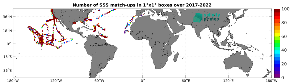
Figure 5: Number of SSS match-ups between Sailability SSS and the SMOS SSS L2 v700 (ESA) SSS product for the Mid-Low Latitudes 45N-45S Pi-MEP region over 1^\circ \times 1^\circ boxes and for the full satellite product period.
