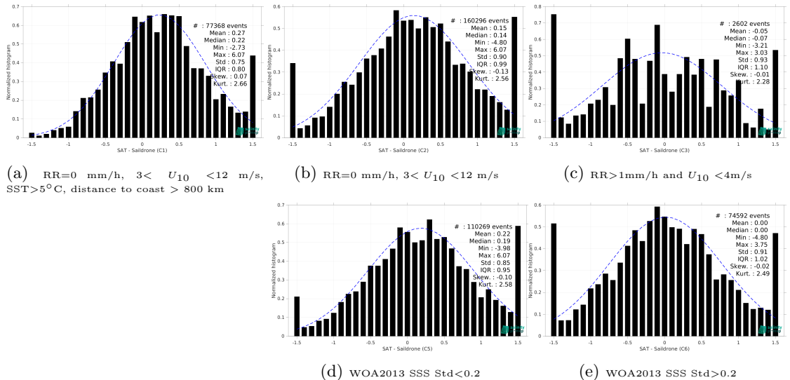
Figure 13: Normalized histogram of \Delta SSS (SMOS SSS L2 v700 (ESA) - Saildrone) for 5 different subdatasets corresponding to: RR=0 mm/h, 3 < U_{10} < 12 m/s, SST>5°C, distance to coast > 800 km (a), RR=0 mm/h, 3 < U_{10} < 12 m/s (b), RR>1mm/h and U_{10} < 4 m/s (c), WOA2013 SSS Std<0.2 (d), WOA2013 SSS Std>0.2 (e).
