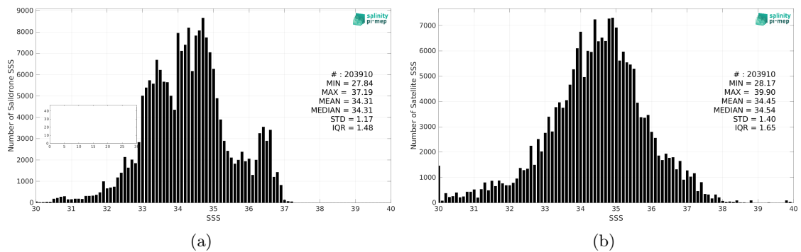
Figure 2: Histograms of SSS from Saildrone (a) and SMOS SSS L2 v700 (ESA) (b) considering all match-up pairs per bins of 0.1 over the Mid-Low Latitudes 45N-45S Pi-MEP region and for the full satellite product period.
