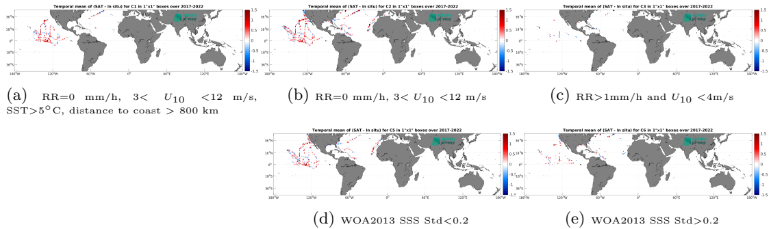
Figure 12: Temporal mean gridded over spatial boxes of size 1^\circ \times 1^\circ of \Delta SSS (SMOS SSS L2 v700 (ESA) - Saildrone) for 5 different subdatasets corresponding to:RR=0 mm/h, 3 < U_{10} < 12 m/s, SST>5°C, distance to coast > 800 km (a), RR=0 mm/h, 3 < U_{10} < 12 m/s (b), RR>1mm/h and U_{10} < 4 m/s (c), WOA2013 SSS Std<0.2 (d), WOA2013 SSS Std>0.2 (e).
