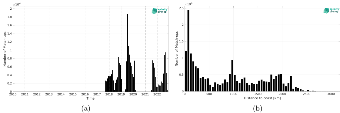
Figure 1: Number of match-ups between Saildrone and SMOS SSS L2 v700 (ESA) SSS as a function of time (a) and as function of the distance to coast (b) over the Mid-Low Latitudes 45N-45S Pi-MEP region and for the full satellite product period.
