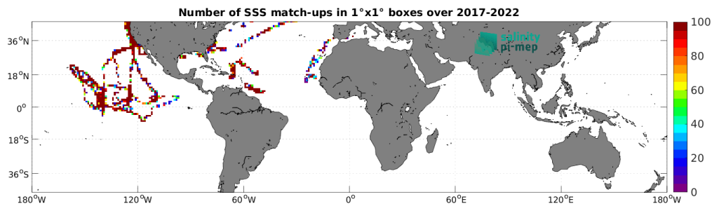
Figure 4: Number of SSS match-ups between Saildrone SSS and the SMOS SSS L2 v700 (ESA) SSS product for the Mid-Low Latitudes 45N-45S Pi-MEP region over 1^\circ \times 1^\circ boxes and for the full satellite product period.
