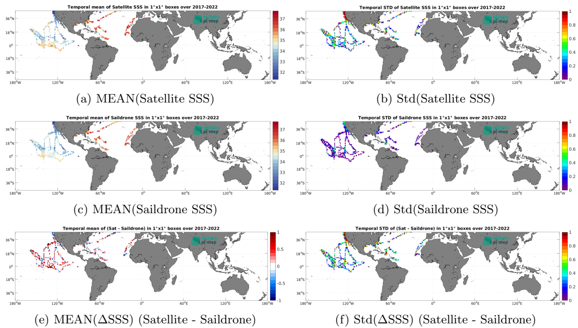
Figure 6: Temporal mean (left) and Std (right) of SSS from SMOS SSS L2 v700 (ESA) (top), Saildrone (middle), and of \Delta SSS (Satellite - Saildrone). Only match-up pairs are used to generate these maps.
