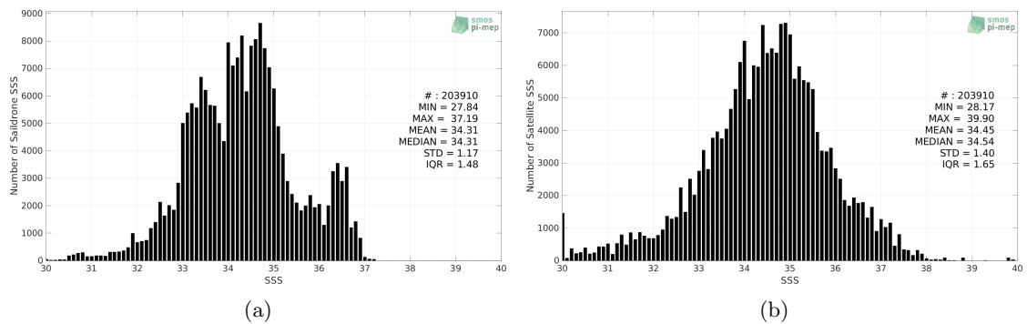
Figure 2: Histograms of SSS from Sairdrone (a) and SMOS SSS L2 v700 (ESA) (b) considering all match-up pairs per bins of 0.1 over the Mid-Low Latitudes 45N-45S Pi-MEP region and for the full satellite product period.
