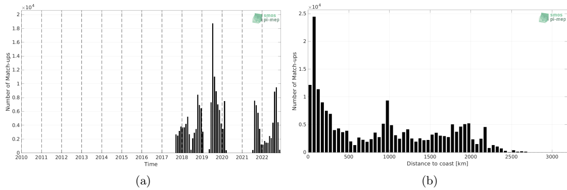
Figure 1: Number of match-ups between Sairdrone and SMOS SSS L2 v700 (ESA) SSS as a function of time (a) and as function of the distance to coast (b) over the Mid-Low Latitudes 45N-45S Pi-MEP region and for the full satellite product period.
