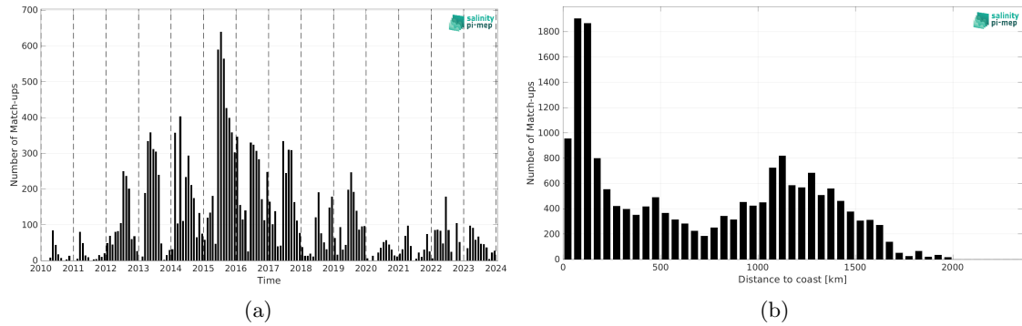
Figure 2: Number of match-ups between Marine mammals and SMOS SSS L2 v700 (ESA) SSS as a function of time (a) and as function of the distance to coast (b) over the Mid-Low Latitudes 45N-45S Pi-MEP region and for the full satellite product period.
