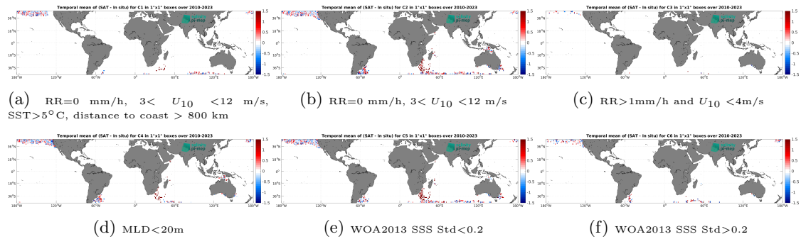
Figure 14: Temporal mean gridded over spatial boxes of size 1^\circ \times 1^\circ of \Delta SSS (SMOS SSS L2 v700 (ESA) - Marine mammals) for 6 different subdatasets corresponding to: RR=0 mm/h, 3 < U_{10} < 12 m/s, SST > 5°C, distance to coast > 800 km (a), RR=0 mm/h, 3 < U_{10} < 12 m/s (b), RR > 1mm/h and U_{10} < 4 m/s (c), MLD < 20m (d), WOA2013 SSS Std < 0.2 (e), WOA2013 SSS Std > 0.2 (f).
