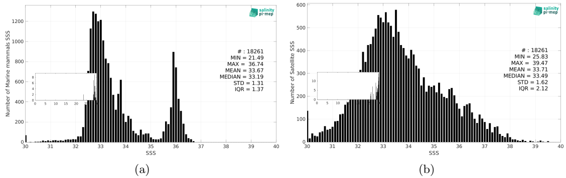
Figure 3: Histograms of SSS from Marine mammals (a) and SMOS SSS L2 v700 (ESA) (b) considering all match-up pairs per bins of 0.1 over the Mid-Low Latitudes 45N-45S Pi-MEP region and for the full satellite product period.
