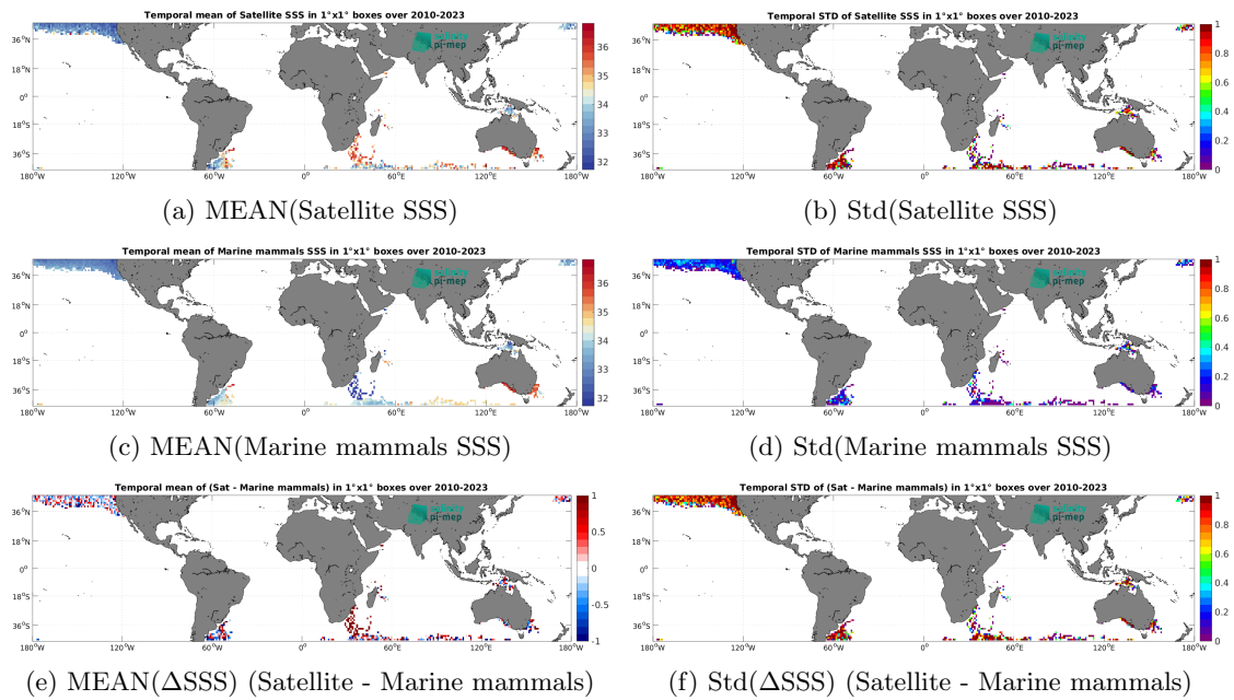
Figure 7: Temporal mean (left) and Std (right) of SSS from SMOS SSS L2 v700 (ESA) (top), Marine mammals (middle), and of \Delta SSS (Satellite - Marine mammals). Only match-up pairs are used to generate these maps.
