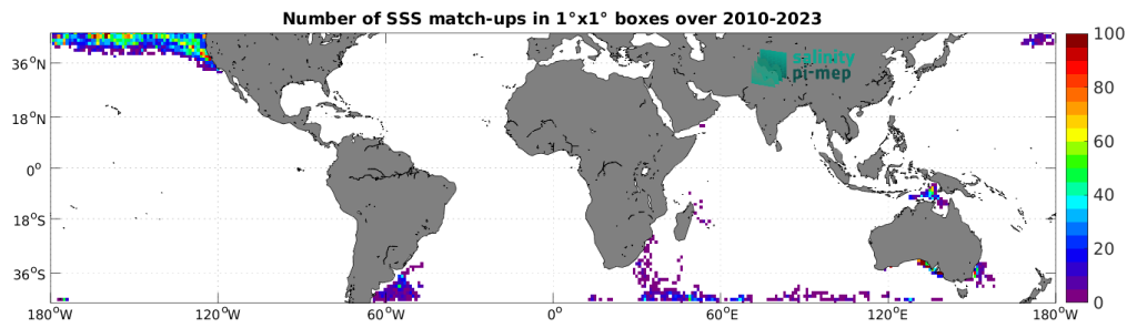
Figure 5: Number of SSS match-ups between Marine mammals SSS and the SMOS SSS L2 v700 (ESA) SSS product for the Mid-Low Latitudes 45N-45S Pi-MEP region over 1^\circ \times 1^\circ boxes and for the full satellite product period.
