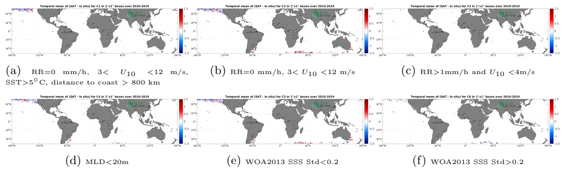
Figure 12: Temporal mean gridded over spatial boxes of size 1^\circ \times 1^\circ of \Delta SSS (SMOS SSS L2 v700 (ESA) - Marine mammals) for 6 different subdatasets corresponding to:RR=0 mm/h, 3 < U_{10} < 12 m/s, SST>5°C, distance to coast > 800 km (a), RR=0 mm/h, 3 < U_{10} < 12 m/s (b), RR>1mm/h and U_{10} < 4 m/s (c),MLD<20m (d),WOA2013 SSS Std<0.2 (e),WOA2013 SSS Std>0.2 (f).
