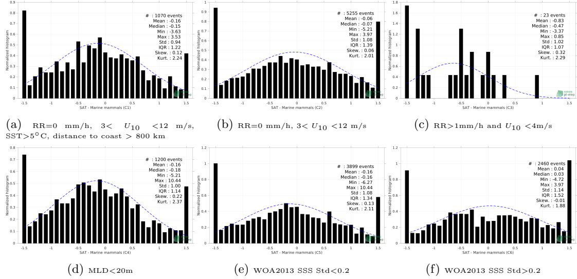
Figure 13: Normalized histogram of \Delta SSS (SMOS SSS L2 v700 (ESA) - Marine mammals) for 6 different subdatasets corresponding to: RR=0 mm/h, 3 < U_{10} < 12 m/s, SST>5°C, distance to coast > 800 km (a), RR=0 mm/h, 3 < U_{10} < 12 m/s (b), RR>1mm/h and U_{10} < 4 m/s (c), MLD<20m (d), WOA2013 SSS Std<0.2 (e), WOA2013 SSS Std>0.2 (f).
