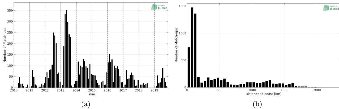
Figure 1: Number of match-ups between Marine mammals and SMOS SSS L2 v700 (ESA) SSS as a function of time (a) and as function of the distance to coast (b) over the Mid-Low Latitudes 45N-45S Pi-MEP region and for the full satellite product period.
