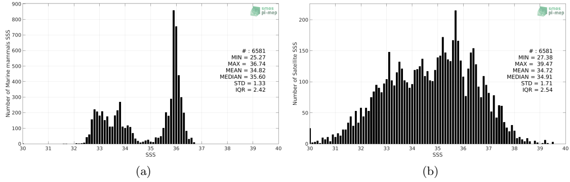
Figure 2: Histograms of SSS from Marine mammals (a) and SMOS SSS L2 v700 (ESA) (b) considering all match-up pairs per bins of 0.1 over the Mid-Low Latitudes 45N-45S Pi-MEP region and for the full satellite product period.
