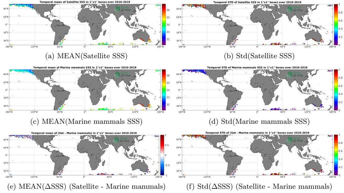
Figure 6: Temporal mean (left) and Std (right) of SSS from SMOS SSS L2 v700 (ESA) (top), Marine mammals (middle), and of \Delta SSS (Satellite - Marine mammals). Only match-up pairs are used to generate these maps.
