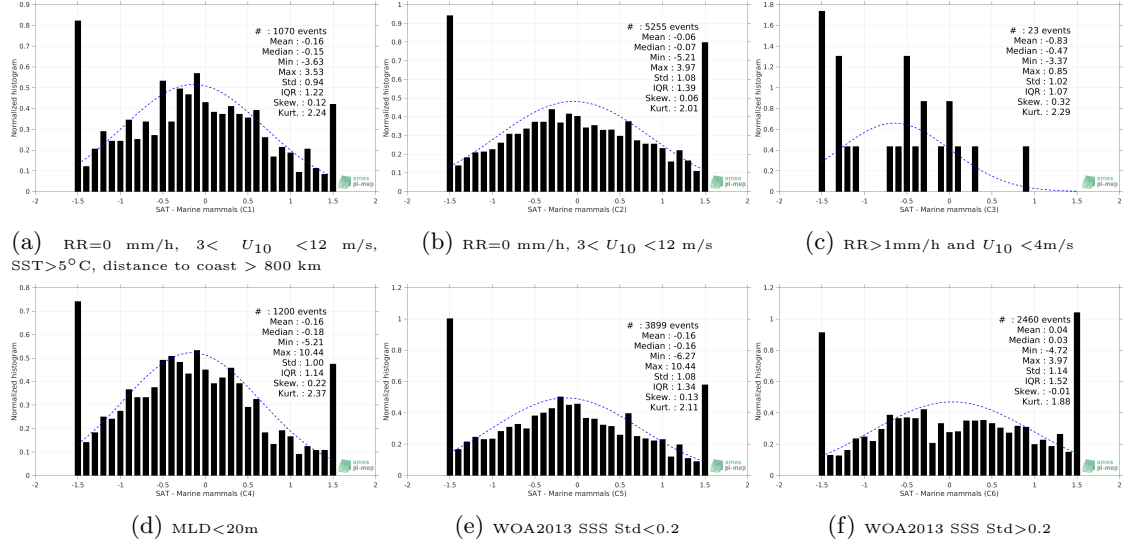
Figure 13: Normalized histogram of \Delta\text{SSS} (SMOS SSS L2 v700 (ESA) - Marine mammals) for 6 different subdatasets corresponding to: RR=0 mm/h, 3 < U_{10} < 12 m/s, SST>5°C, distance to coast > 800 km (a), RR=0 mm/h, 3 < U_{10} < 12 m/s (b), RR>1mm/h and U_{10} < 4 m/s (c), MLD<20m (d), WOA2013 SSS Std<0.2 (e), WOA2013 SSS Std>0.2 (f).
