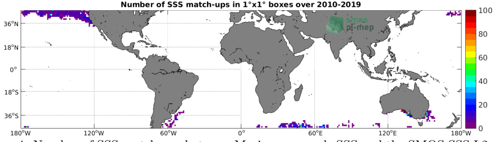
Figure 4: Number of SSS match-ups between Marine mammals SSS and the SMOS SSS L2 v700 (ESA) SSS product for the Mid-Low Latitudes 45N-45S Pi-MEP region over 1^\circ \times 1^\circ boxes and for the full satellite product period.
