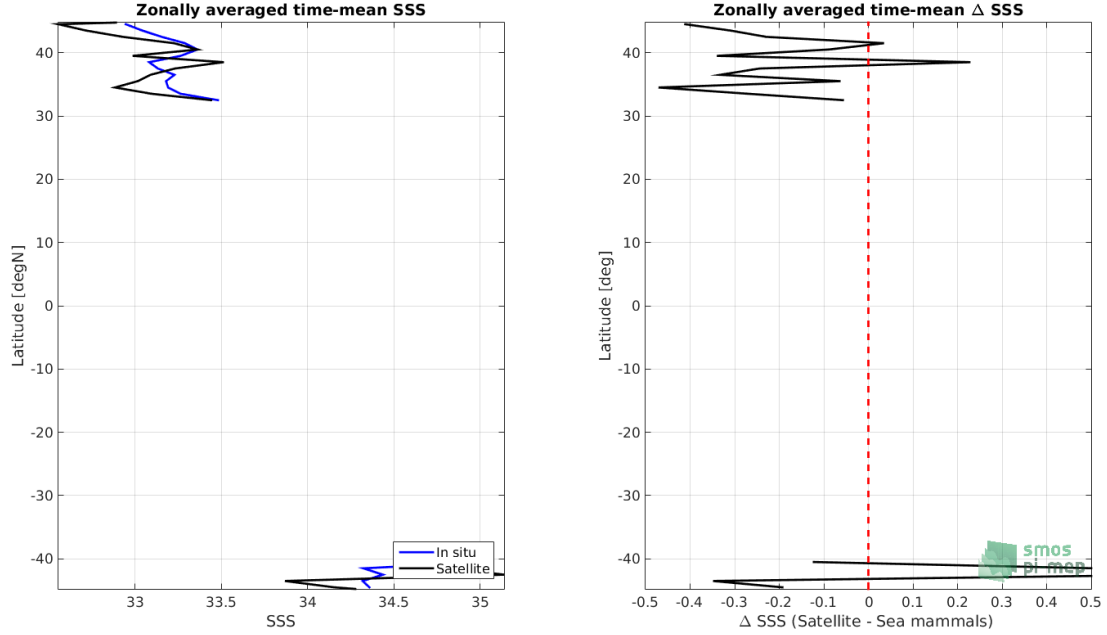
Figure 8: Left panel: Zonal mean SSS from SMOS SSS L2 v700 (ESA) satellite product (black) and from Sea mammals (blue). Right panel: Zonal mean of \Delta SSS (Satellite - Sea mammals) for all the collected Pi-MEP match-up pairs estimated over the full satellite product period.
