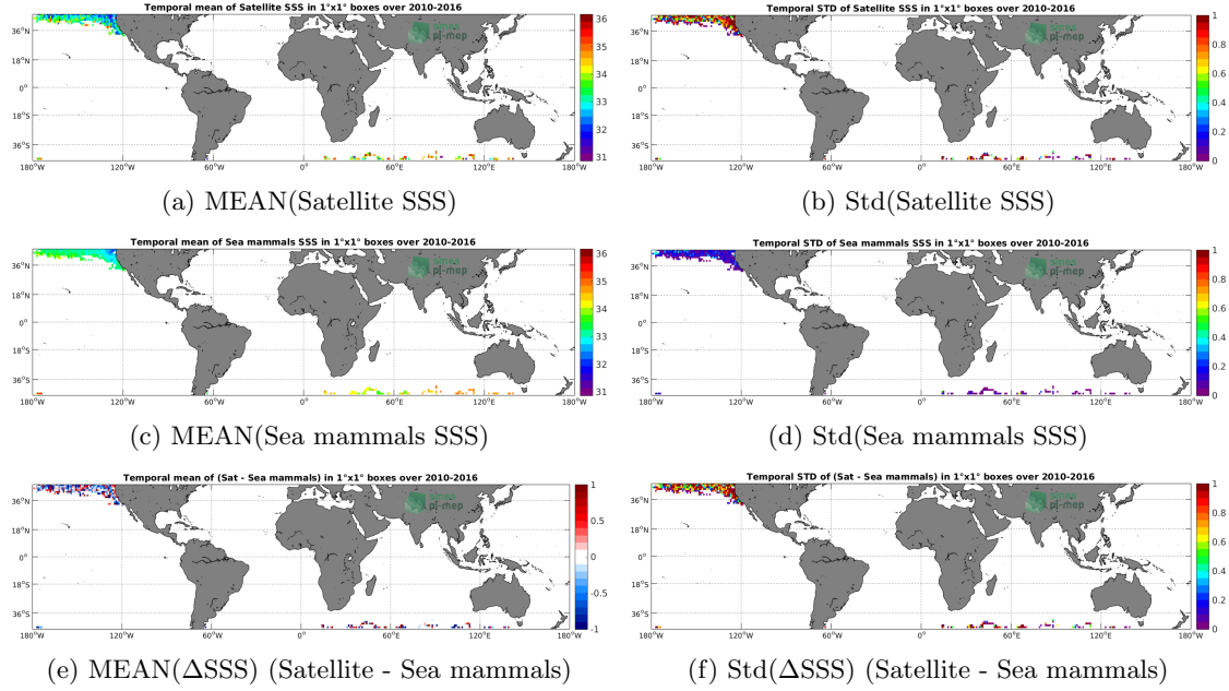
Figure 6: Temporal mean (left) and Std (right) of SSS from SMOS SSS L2 v700 (ESA) (top), Sea mammals (middle), and of \Delta SSS (Satellite - Sea mammals). Only match-up pairs are used to generate these maps.
