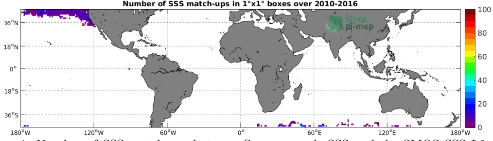
Figure 4: Number of SSS match-ups between Sea mammals SSS and the SMOS SSS L2 v700 (ESA) SSS product for the Mid-Low Latitudes 45N-45S Pi-MEP region over 1°x1° boxes and for the full satellite product period.
