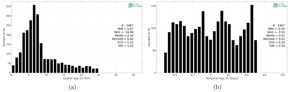
Figure 5: Histograms of the spatial (a) and temporal (b) lags between the location/time of the Sea mammals measurement and the date of the corresponding SMOS SSS L2 v700 (ESA) SSS pixel.
