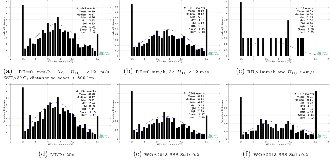
Figure 13: Normalized histogram of \Delta\text{SSS} (SMOS SSS L2 v700 (ESA) - Sea mammals) for 6 different subdatasets corresponding to: RR=0 mm/h, 3 < U_{10} < 12 m/s, SST>5°C, distance to coast > 800 km (a), RR=0 mm/h, 3 < U_{10} < 12 m/s (b), RR>1mm/h and U_{10} < 4 m/s (c), MLD<20m (d), WOA2013 SSS Std<0.2 (e), WOA2013 SSS Std>0.2 (f).
