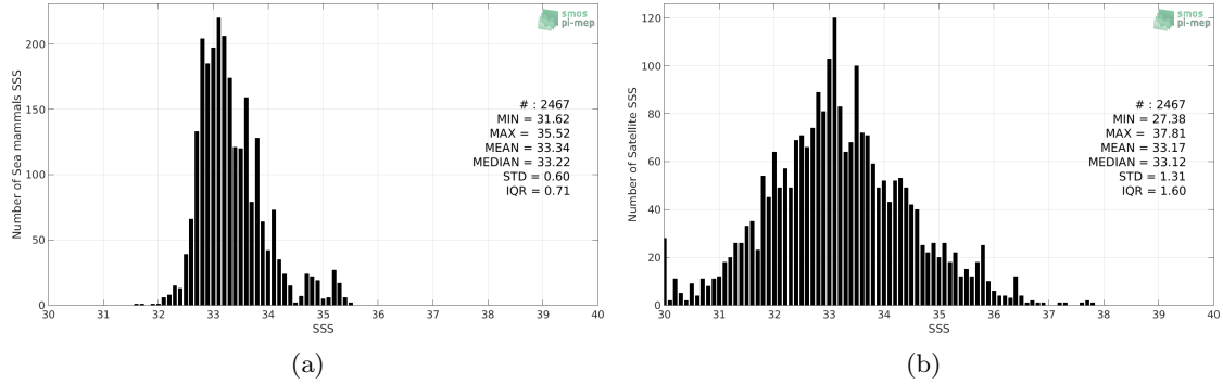
Figure 2: Histograms of SSS from Sea mammals (a) and SMOS SSS L2 v700 (ESA) (b) considering all match-up pairs per bins of 0.1 over the Mid-Low Latitudes 45N-45S Pi-MEP region and for the full satellite product period.
