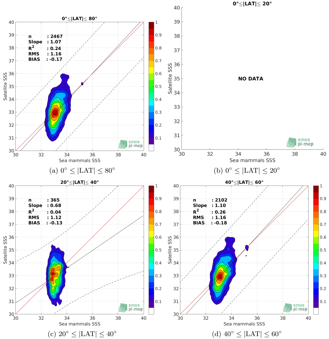
Figure 9: Contour maps of the concentration of SMOS SSS L2 v700 (ESA) SSS (y-axis) versus Sea mammals SSS (x-axis) at match-up pairs for different latitude bands. For each plot, the red line shows x=y . The black thin and dashed lines indicate a linear fit through the data cloud and the \pm 95\% confidence levels, respectively. The number match-up pairs n , the slope and R^2 coefficient of the linear fit, the root mean square (RMS) and the mean bias between satellite and in situ data are indicated for each latitude band in each plots.
