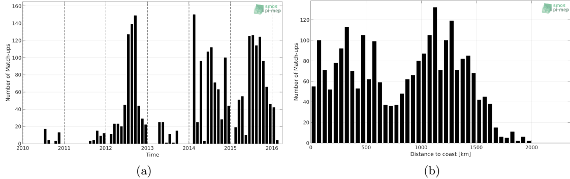
Figure 1: Number of match-ups between Sea mammals and SMOS SSS L2 v700 (ESA) SSS as a function of time (a) and as function of the distance to coast (b) over the Mid-Low Latitudes 45N-45S Pi-MEP region and for the full satellite product period.
