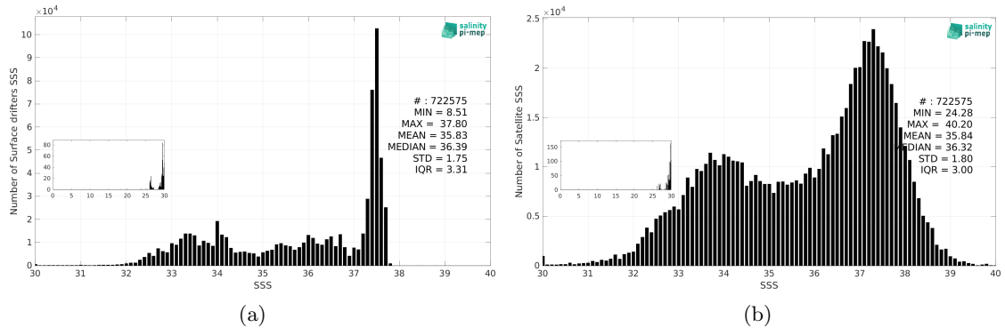
Figure 3: Histograms of SSS from Surface drifters (a) and SMOS SSS L2 v700 (ESA) (b) considering all match-up pairs per bins of 0.1 over the Mid-Low Latitudes 45N-45S Pi-MEP region and for the full satellite product period.
