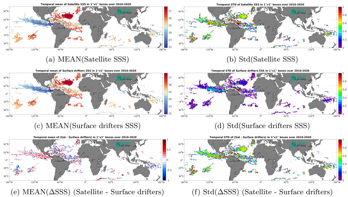
Figure 6: Temporal mean (left) and Std (right) of SSS from SMOS SSS L2 v700 (ESA) (top), Surface drifters (middle), and of \Delta SSS (Satellite - Surface drifters). Only match-up pairs are used to generate these maps.
