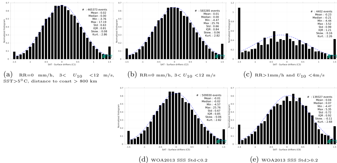
Figure 14: Normalized histogram of \Delta SSS (SMOS SSS L2 v700 (ESA) - Surface drifters) for 5 different subdatasets corresponding to: RR=0 mm/h, 3 < U_{10} < 12 m/s, SST >5^\circ\text{C} , distance to coast > 800 km (a), RR=0 mm/h, 3 < U_{10} < 12 m/s (b), RR >1 mm/h and U_{10} < 4 m/s (c), WOA2013 SSS Std <0.2 (d), WOA2013 SSS Std >0.2 (e).
