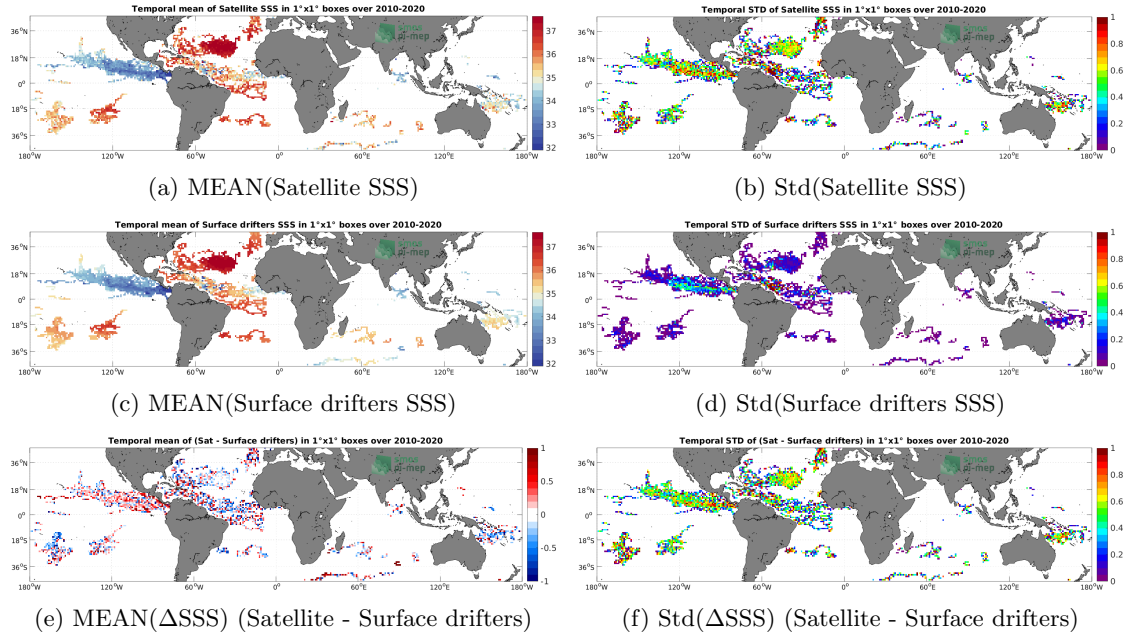
Figure 5: Temporal mean (left) and Std (right) of SSS from SMOS SSS L2 v700 (ESA) (top), Surface drifters (middle), and of \Delta SSS (Satellite - Surface drifters). Only match-up pairs are used to generate these maps.
