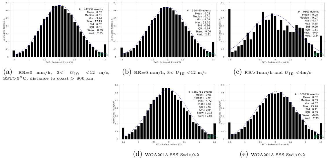
Figure 12: Normalized histogram of \Delta SSS (SMOS SSS L2 v700 (ESA) - Surface drifters) for 5 different subdatasets corresponding to: RR=0 mm/h, 3 < U_{10} < 12 m/s, SST >5^\circ\text{C} , distance to coast > 800 km (a), RR=0 mm/h, 3 < U_{10} < 12 m/s (b), RR >1 mm/h and U_{10} < 4 m/s (c), WOA2013 SSS Std <0.2 (d), WOA2013 SSS Std >0.2 (e).
