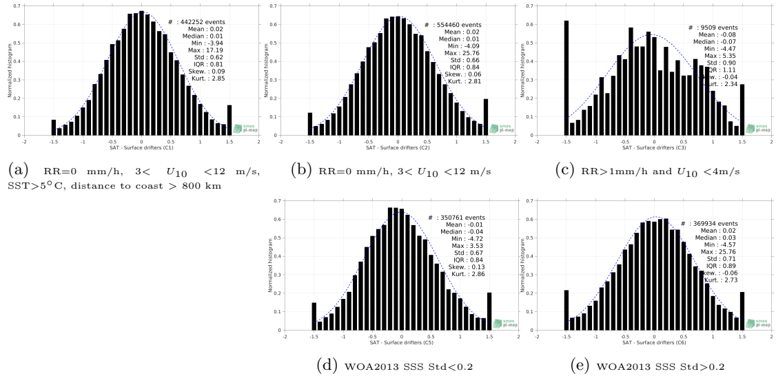
Figure 12: Normalized histogram of \Delta\text{SSS} (SMOS SSS L2 v700 (ESA) - Surface drifters) for 5 different subdatasets corresponding to: \text{RR}=0 mm/h, 3 < U_{10} < 12 m/s, \text{SST}>5^\circ\text{C} , distance to coast > 800 km (a), \text{RR}=0 mm/h, 3 < U_{10} < 12 m/s (b), \text{RR}>1\text{mm/h} and U_{10} < 4\text{m/s} (c), WOA2013 SSS Std <0.2 (d), WOA2013 SSS Std >0.2 (e).
