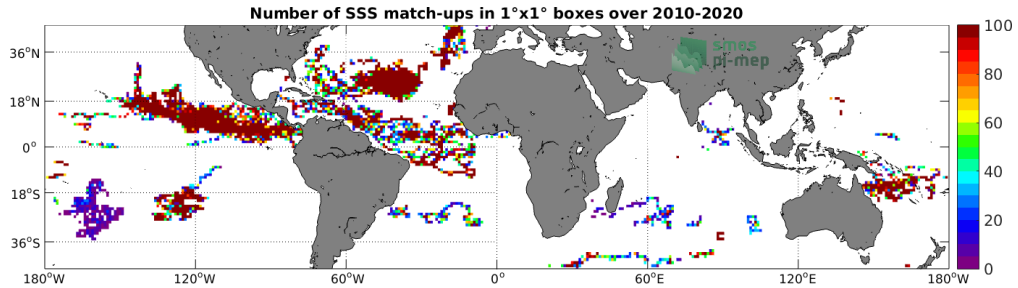
Figure 3: Number of SSS match-ups between Surface drifters SSS and the SMOS SSS L2 v700 (ESA) SSS product for the Mid-Low Latitudes 45N-45S Pi-MEP region over 1^\circ \times 1^\circ boxes and for the full satellite product period.
