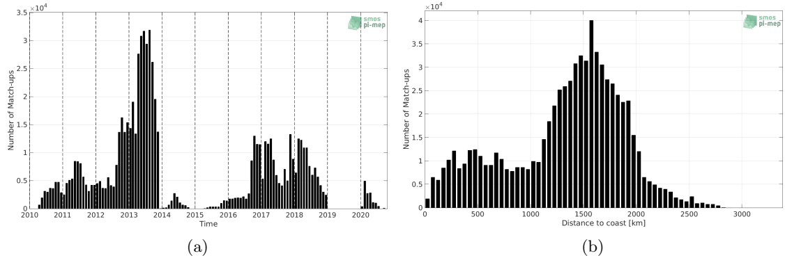
Figure 1: Number of match-ups between Surface drifters and SMOS SSS L2 v700 (ESA) SSS as a function of time (a) and as function of the distance to coast (b) over the Mid-Low Latitudes 45N-45S Pi-MEP region and for the full satellite product period.
