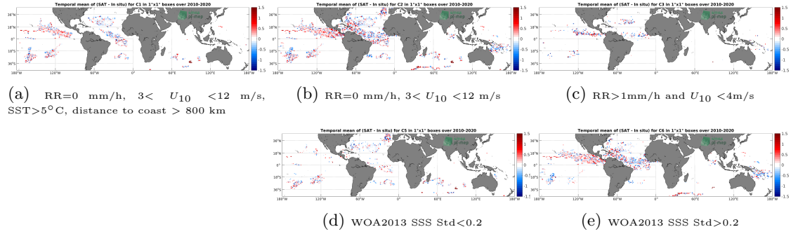
Figure 11: Temporal mean gridded over spatial boxes of size 1^\circ \times 1^\circ of \Delta\text{SSS} (SMOS SSS L2 v700 (ESA) - Surface drifters) for 5 different subdatasets corresponding to: \text{RR}=0 mm/h, 3 < U_{10} < 12 m/s, \text{SST}>5^\circ\text{C} , distance to coast > 800 km (a), \text{RR}=0 mm/h, 3 < U_{10} < 12 m/s (b), \text{RR}>1\text{mm/h} and U_{10} < 4\text{m/s} (c), WOA2013 SSS Std <0.2 (d), WOA2013 SSS Std >0.2 (e).
