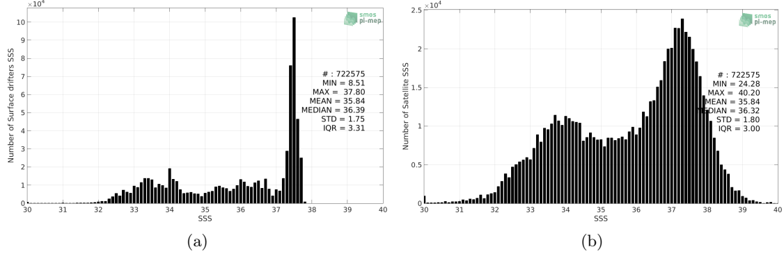
Figure 2: Histograms of SSS from Surface drifters (a) and SMOS SSS L2 v700 (ESA) (b) considering all match-up pairs per bins of 0.1 over the Mid-Low Latitudes 45N-45S Pi-MEP region and for the full satellite product period.
