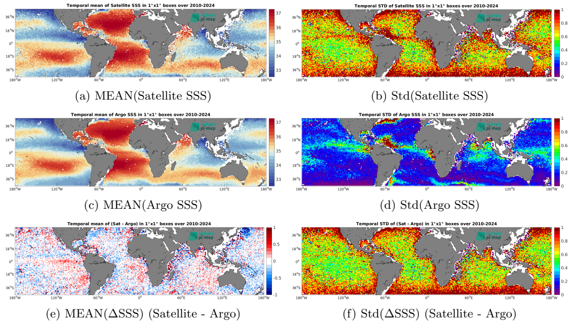
Figure 7: Temporal mean (left) and Std (right) of SSS from SMOS SSS L2 v700 (ESA) (top), Argo (middle), and of \Delta SSS (Satellite - Argo). Only match-up pairs are used to generate these maps.
