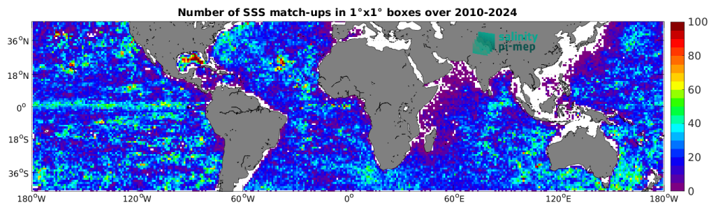
Figure 5: Number of SSS match-ups between Argo SSS and the SMOS SSS L2 v700 (ESA) SSS product for the Mid-Low Latitudes 45N-45S Pi-MEP region over 1^\circ \times 1^\circ boxes and for the full satellite product period.
