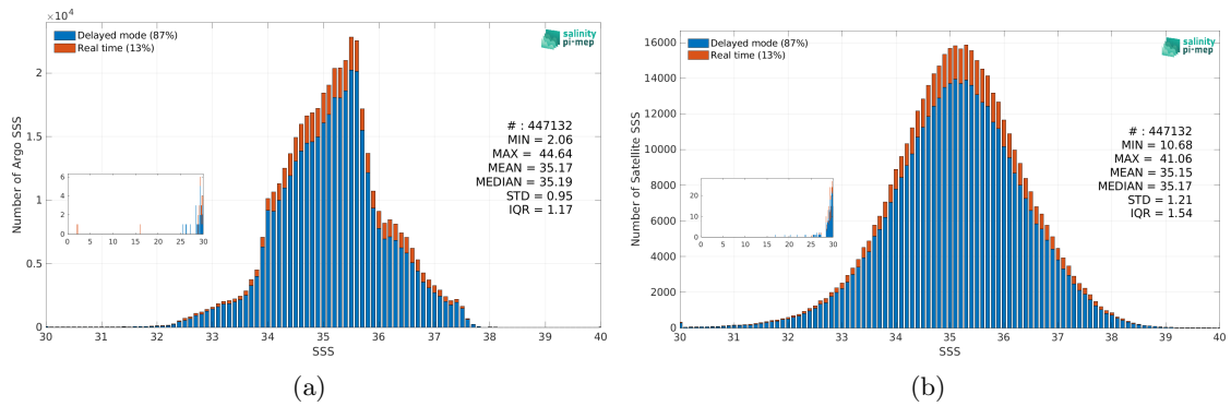
Figure 3: Histograms of SSS from Argo (a) and SMOS SSS L2 v700 (ESA) (b) considering all match-up pairs per bins of 0.1 over the Mid-Low Latitudes 45N-45S Pi-MEP region and for the full satellite product period.
