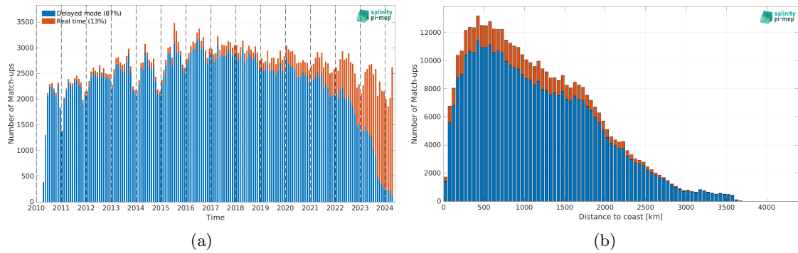
Figure 2: Number of match-ups between Argo and SMOS SSS L2 v700 (ESA) SSS as a function of time (a) and as function of the distance to coast (b) over the Mid-Low Latitudes 45N-45S Pi-MEP region and for the full satellite product period.
