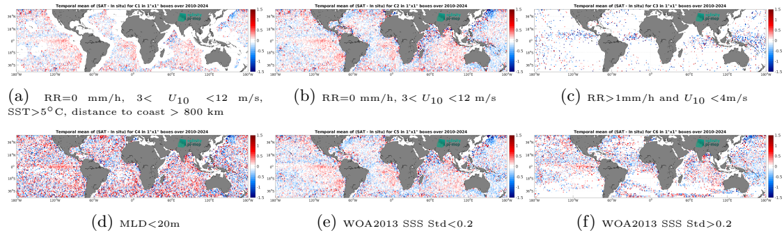
Figure 14: Temporal mean gridded over spatial boxes of size 1^\circ \times 1^\circ of \Delta SSS (SMOS SSS L2 v700 (ESA) - Argo) for 6 different subdatasets corresponding to:RR=0 mm/h, 3 < U_{10} < 12 m/s, SST>5°C, distance to coast > 800 km (a), RR=0 mm/h, 3 < U_{10} < 12 m/s (b), RR>1mm/h and U_{10} < 4 m/s (c),MLD<20m (d),WOA2013 SSS Std<0.2 (e),WOA2013 SSS Std>0.2 (f).
