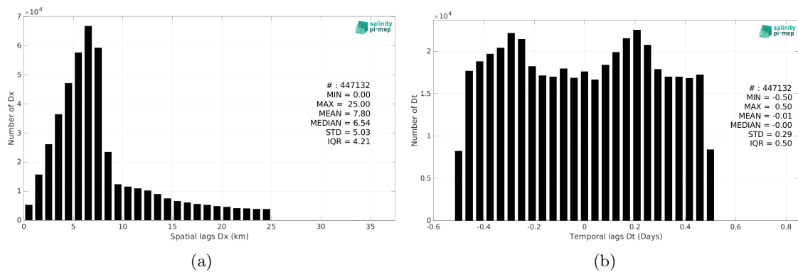
Figure 6: Histograms of the spatial (a) and temporal (b) lags between the location/time of the Argo measurement and the date of the corresponding SMOS SSS L2 v700 (ESA) SSS pixel.
