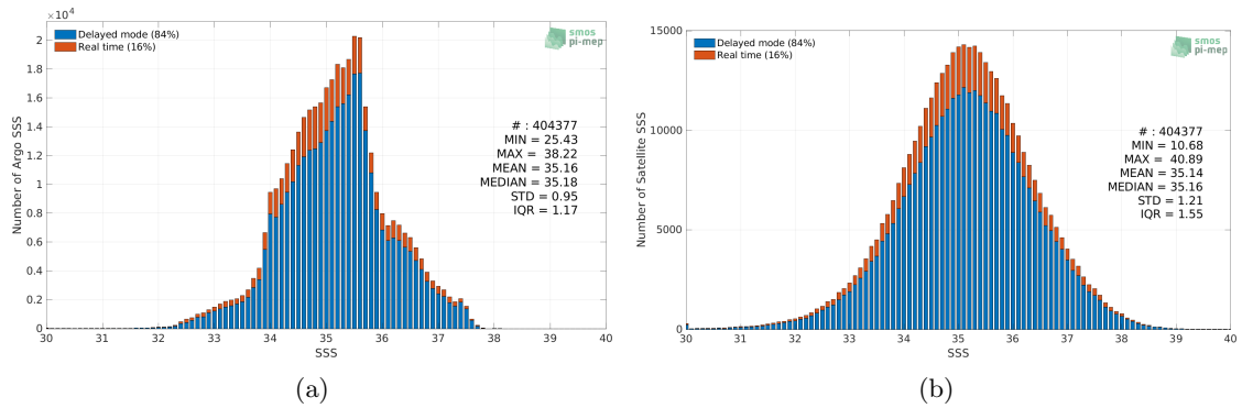
Figure 2: Histograms of SSS from Argo (a) and SMOS SSS L2 v700 (ESA) (b) considering all match-up pairs per bins of 0.1 over the Mid-Low Latitudes 45N-45S Pi-MEP region and for the full satellite product period.
