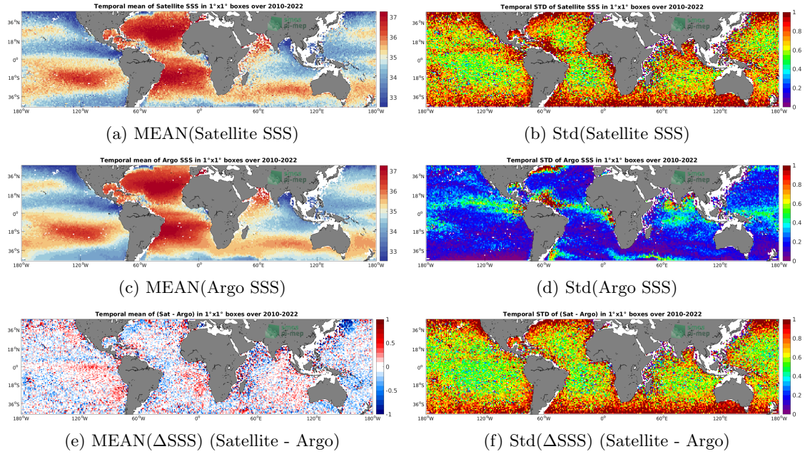
Figure 6: Temporal mean (left) and Std (right) of SSS from SMOS SSS L2 v700 (ESA) (top), Argo (middle), and of \Delta SSS (Satellite - Argo). Only match-up pairs are used to generate these maps.
