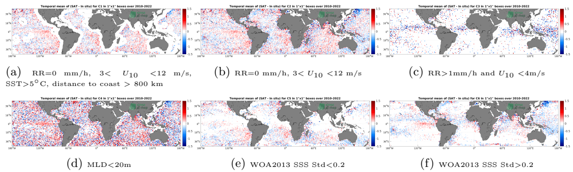
Figure 12: Temporal mean gridded over spatial boxes of size 1^\circ \times 1^\circ of \Delta SSS (SMOS SSS L2 v700 (ESA) - Argo) for 6 different subdatasets corresponding to:RR=0 mm/h, 3 < U_{10} < 12 m/s, SST >5^\circ C, distance to coast > 800 km (a), RR=0 mm/h, 3 < U_{10} < 12 m/s (b), RR >1 mm/h and U_{10} < 4 m/s (c),MLD <20 m (d),WOA2013 SSS Std <0.2 (e),WOA2013 SSS Std >0.2 (f).
