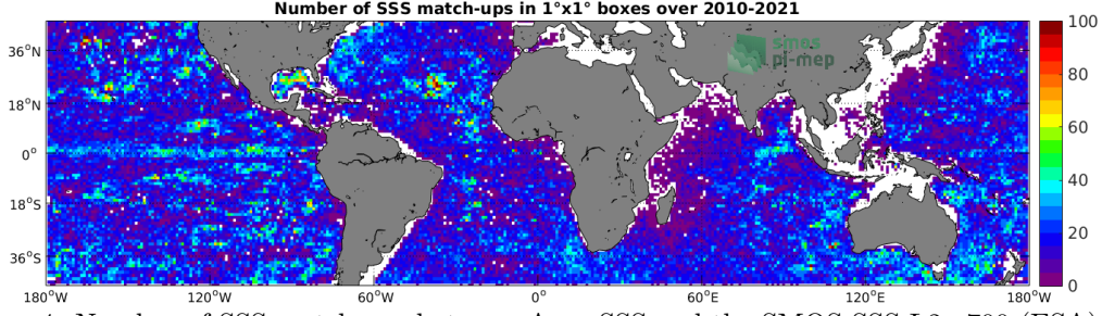
Figure 4: Number of SSS match-ups between Argo SSS and the SMOS SSS L2 v700 (ESA) SSS product for the Mid-Low Latitudes 45N-45S Pi-MEP region over 1^\circ \times 1^\circ boxes and for the full satellite product period.
