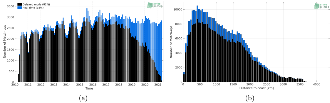
Figure 1: Number of match-ups between Argo and SMOS SSS L2 v700 (ESA) SSS as a function of time (a) and as function of the distance to coast (b) over the Mid-Low Latitudes 45N-45S Pi-MEP region and for the full satellite product period.
