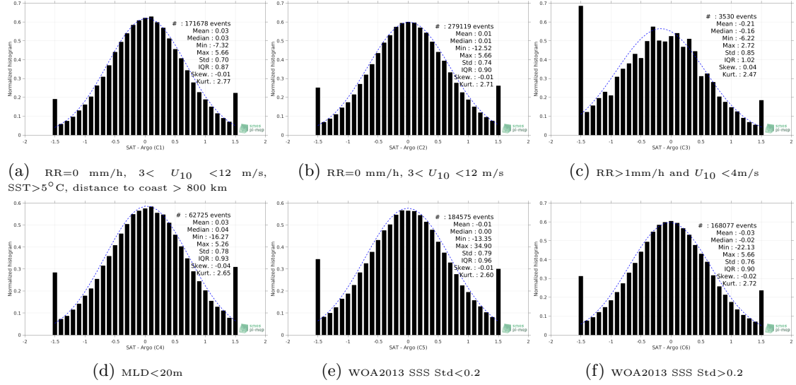
Figure 13: Normalized histogram of \Delta\text{SSS} (SMOS SSS L2 v700 (ESA) - Argo) for 6 different subdatasets corresponding to: RR=0 mm/h, 3 < U_{10} < 12 m/s, SST>5°C, distance to coast > 800 km (a), RR=0 mm/h, 3 < U_{10} < 12 m/s (b), RR>1mm/h and U_{10} < 4 m/s (c), MLD<20m (d), WOA2013 SSS Std<0.2 (e), WOA2013 SSS Std>0.2 (f).
