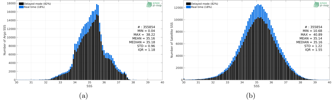
Figure 2: Histograms of SSS from Argo (a) and SMOS SSS L2 v700 (ESA) (b) considering all match-up pairs per bins of 0.1 over the Mid-Low Latitudes 45N-45S Pi-MEP region and for the full satellite product period.
