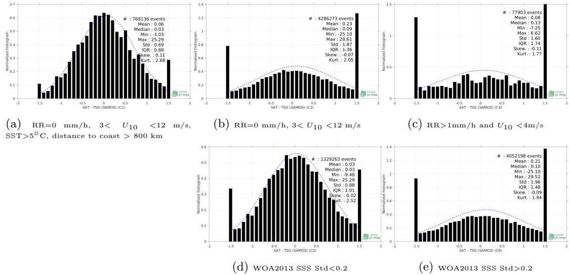
Figure 13: Normalized histogram of \Delta SSS (SMOS SSS L2 v662 (ESA) - TSG (SAMOS)) for 5 different subdatasets corresponding to: RR=0 mm/h, 3 < U_{10} < 12 m/s, SST >5^\circ\text{C} , distance to coast > 800 km (a), RR=0 mm/h, 3 < U_{10} < 12 m/s (b), RR >1 mm/h and U_{10} < 4 m/s (c), WOA2013 SSS Std <0.2 (d), WOA2013 SSS Std >0.2 (e).
