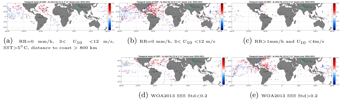
Figure 12: Temporal mean gridded over spatial boxes of size 1^\circ \times 1^\circ of \Delta SSS (SMOS SSS L2 v662 (ESA) - TSG (SAMOS)) for 5 different subdatasets corresponding to: RR=0 mm/h, 3 < U_{10} < 12 m/s, SST >5^\circ\text{C} , distance to coast > 800 km (a), RR=0 mm/h, 3 < U_{10} < 12 m/s (b), RR >1 mm/h and U_{10} < 4 m/s (c), WOA2013 SSS Std <0.2 (d), WOA2013 SSS Std >0.2 (e).
