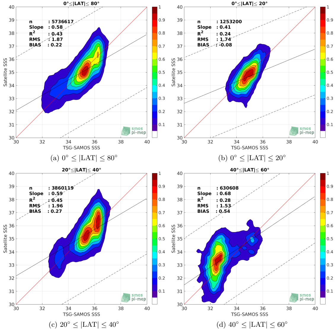
Figure 9: Contour maps of the concentration of SMOS L2 v662 (ESA) SSS (y-axis) versus TSG-SAMOS SSS (x-axis) at match-up pairs for different latitude bands. For each plot, the red line shows x=y . The black thin and dashed lines indicate a linear fit through the data cloud and the \pm 95\% confidence levels, respectively. The number match-up pairs n , the slope and R^2 coefficient of the linear fit, the root mean square (RMS) and the mean bias between satellite and in situ data are indicated for each latitude band in each plots.
