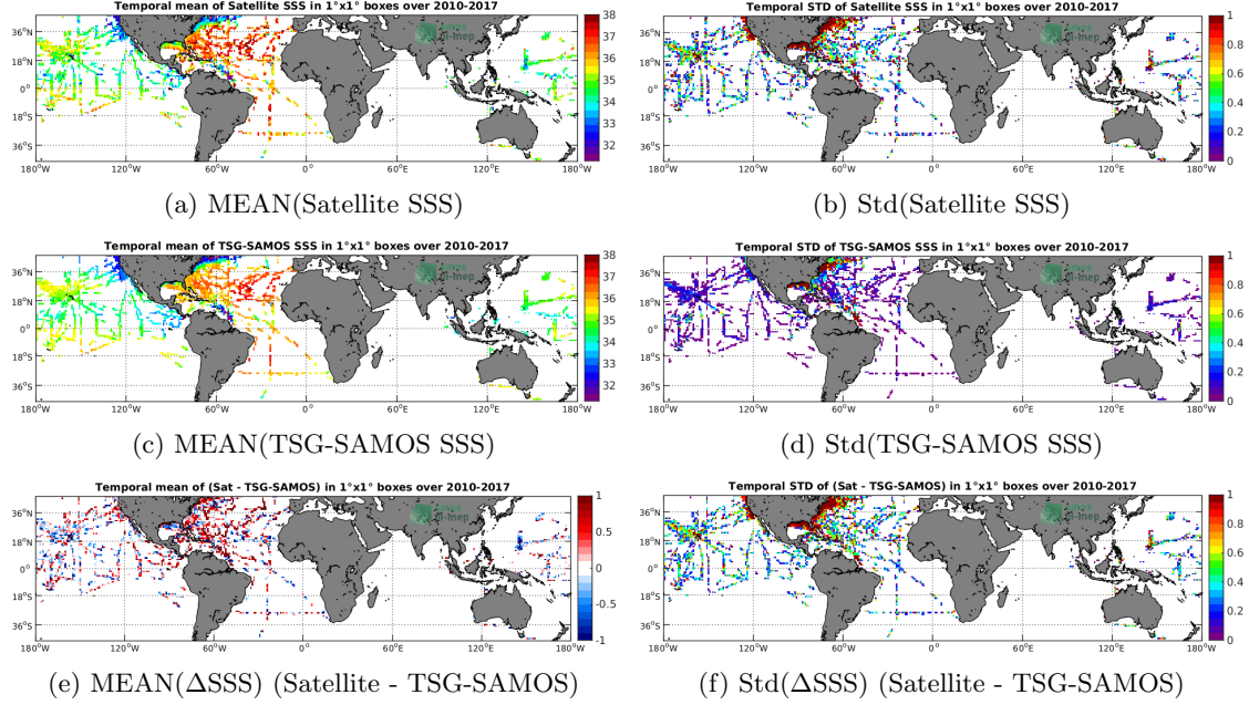
Figure 6: Temporal mean (left) and Std (right) of SSS from SMOS-L2-DPGS-v662 (top), TSG-SAMOS (middle), and of \Delta SSS (Satellite - TSG-SAMOS). Only match-up pairs are used to generate these maps.
