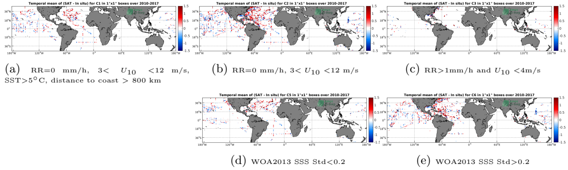
Figure 12: Temporal mean gridded over spatial boxes of size 1^\circ \times 1^\circ of \Delta SSS (SMOS-L2-DPGS-v662 - TSG-SAMOS) for 5 different subdatasets corresponding to:RR=0 mm/h, 3 < U_{10} < 12 m/s, SST >5^\circ\text{C} , distance to coast > 800 km (a), RR=0 mm/h, 3 < U_{10} < 12 m/s (b), RR >1 mm/h and U_{10} < 4 m/s (c), WOA2013 SSS Std <0.2 (d), WOA2013 SSS Std >0.2 (e).
