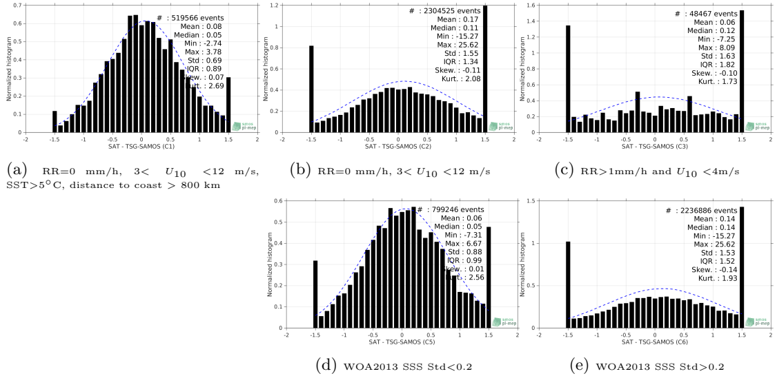
Figure 13: Normalized histogram of \Delta SSS (SMOS-L2-DPGS-v662 - TSG-SAMOS) for 5 different subdatasets corresponding to: RR=0 mm/h, 3 < U_{10} < 12 m/s, SST >5^\circ\text{C} , distance to coast > 800 km (a), RR=0 mm/h, 3 < U_{10} < 12 m/s (b), RR >1 mm/h and U_{10} < 4 m/s (c), WOA2013 SSS Std <0.2 (d), WOA2013 SSS Std >0.2 (e).
