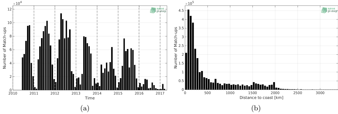
Figure 1: Number of match-ups between TSG-SAMOS and SMOS-L2-DPGS-v662 SSS as a function of time (a) and as function of the distance to coast (b) over the Mid-Low Latitudes 45N-45S Pi-MEP region and for the full satellite product period.
