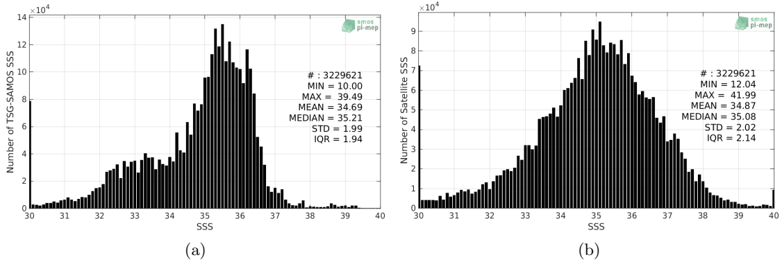
Figure 2: Histograms of SSS from TSG-SAMOS (a) and SMOS-L2-DPGS-v662 (b) considering all match-up pairs per bins of 0.1 over the Mid-Low Latitudes 45N-45S Pi-MEP region and for the full satellite product period.
