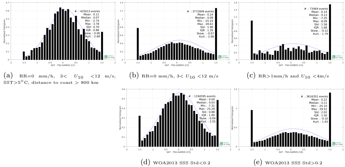
Figure 13: Normalized histogram of \Delta SSS (SMOS-L2-DPGS-v662 - TSG-SAMOS) for 5 different subdatasets corresponding to: RR=0 mm/h, 3 < U_{10} < 12 m/s, SST > 5^\circ C , distance to coast > 800 km (a), RR=0 mm/h, 3 < U_{10} < 12 m/s (b), RR > 1 mm/h and U_{10} < 4 m/s (c), WOA2013 SSS Std < 0.2 (d), WOA2013 SSS Std > 0.2 (e).
