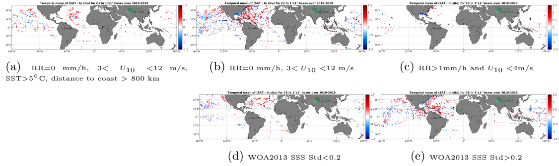
Figure 12: Temporal mean gridded over spatial boxes of size 1^\circ \times 1^\circ of \Delta SSS (SMOS-L2-DPGS-v662 - TSG-SAMOS) for 5 different subdatasets corresponding to: RR=0 mm/h, 3 < U_{10} < 12 m/s, SST > 5^\circ C , distance to coast > 800 km (a), RR=0 mm/h, 3 < U_{10} < 12 m/s (b), RR > 1 mm/h and U_{10} < 4 m/s (c), WOA2013 SSS Std < 0.2 (d), WOA2013 SSS Std > 0.2 (e).
