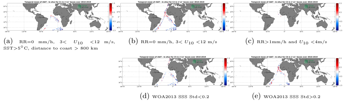
Figure 12: Temporal mean gridded over spatial boxes of size 1^\circ \times 1^\circ of \Delta SSS (SMOS SSS L2 v662 (ESA) - TSG (Polarstern)) for 5 different subdatasets corresponding to:RR=0 mm/h, 3 < U_{10} < 12 m/s, SST >5^\circ\text{C} , distance to coast > 800 km (a), RR=0 mm/h, 3 < U_{10} < 12 m/s (b), RR >1 mm/h and U_{10} < 4 m/s (c), WOA2013 SSS Std <0.2 (d), WOA2013 SSS Std >0.2 (e).
