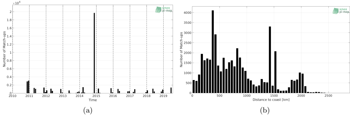
Figure 1: Number of match-ups between TSG (Polarstern) and SMOS SSS L2 v662 (ESA) SSS as a function of time (a) and as function of the distance to coast (b) over the Mid-Low Latitudes 45N-45S Pi-MEP region and for the full satellite product period.
