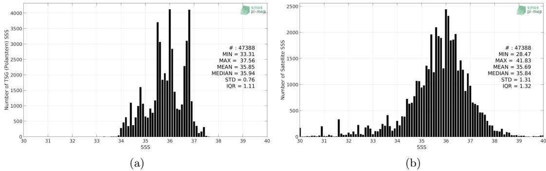
Figure 2: Histograms of SSS from TSG (Polarstern) (a) and SMOS SSS L2 v662 (ESA) (b) considering all match-up pairs per bins of 0.1 over the Mid-Low Latitudes 45N-45S Pi-MEP region and for the full satellite product period.
