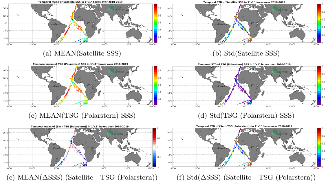
Figure 6: Temporal mean (left) and Std (right) of SSS from SMOS SSS L2 v662 (ESA) (top), TSG (Polarstern) (middle), and of \Delta SSS (Satellite - TSG (Polarstern)). Only match-up pairs are used to generate these maps.
