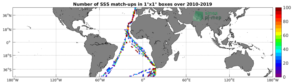
Figure 4: Number of SSS match-ups between TSG (Polarstern) SSS and the SMOS SSS L2 v662 (ESA) SSS product for the Mid-Low Latitudes 45N-45S Pi-MEP region over 1^\circ \times 1^\circ boxes and for the full satellite product period.
