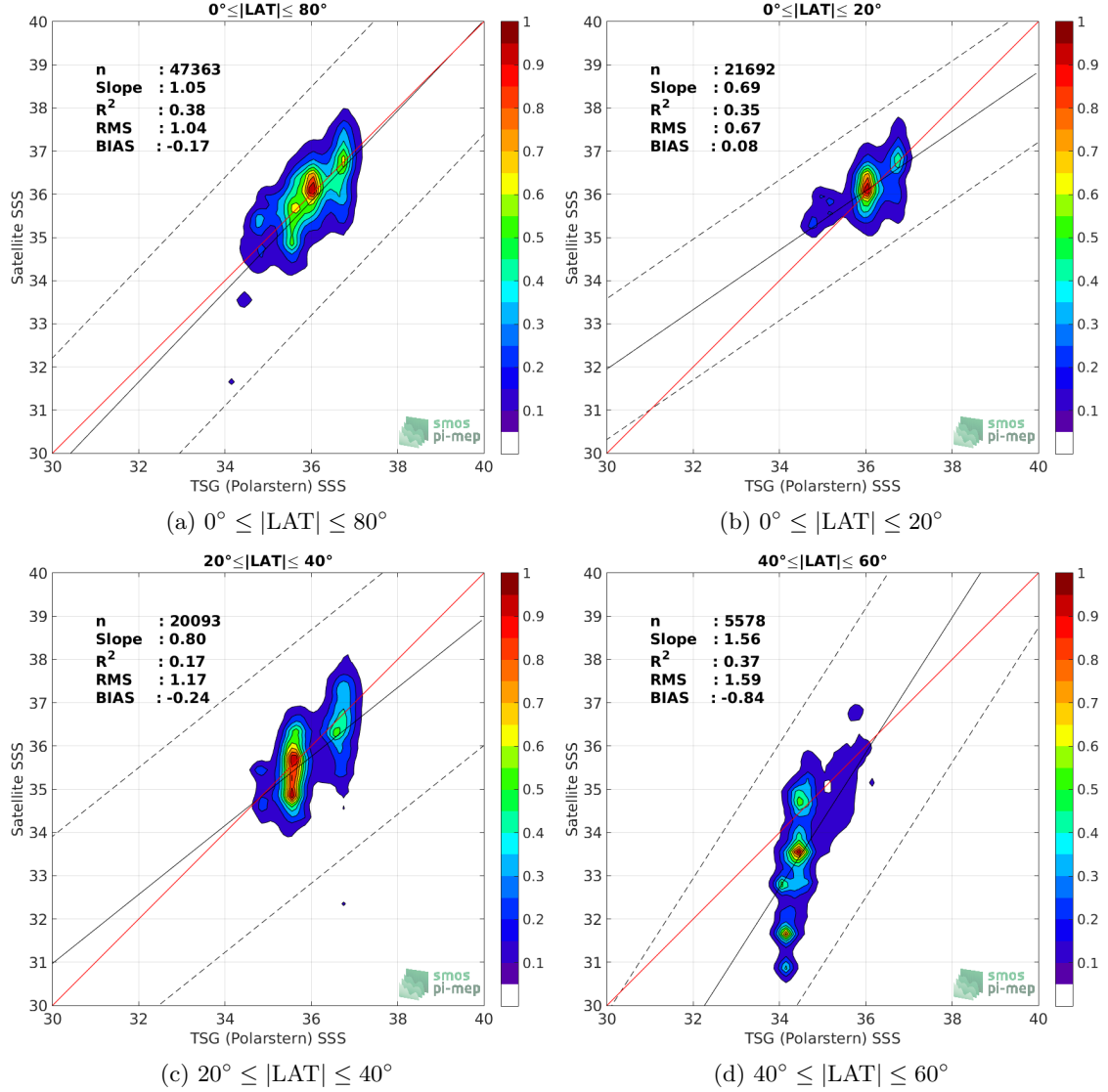
Figure 9: Contour maps of the concentration of SMOS SSS L2 v662 (ESA) SSS (y-axis) versus TSG (Polarstern) SSS (x-axis) at match-up pairs for different latitude bands. For each plot, the red line shows x=y . The black thin and dashed lines indicate a linear fit through the data cloud and the \pm 95\% confidence levels, respectively. The number match-up pairs n , the slope and R^2 coefficient of the linear fit, the root mean square (RMS) and the mean bias between satellite and in situ data are indicated for each latitude band in each plots.
