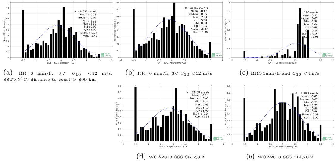
Figure 13: Normalized histogram of \Delta SSS (SMOS SSS L2 v662 (ESA) - TSG (Polarstern)) for 5 different subdatasets corresponding to: RR=0 mm/h, 3 < U_{10} < 12 m/s, SST > 5^\circ C , distance to coast > 800 km (a), RR=0 mm/h, 3 < U_{10} < 12 m/s (b), RR > 1 mm/h and U_{10} < 4 m/s (c), WOA2013 SSS Std < 0.2 (d), WOA2013 SSS Std > 0.2 (e).
