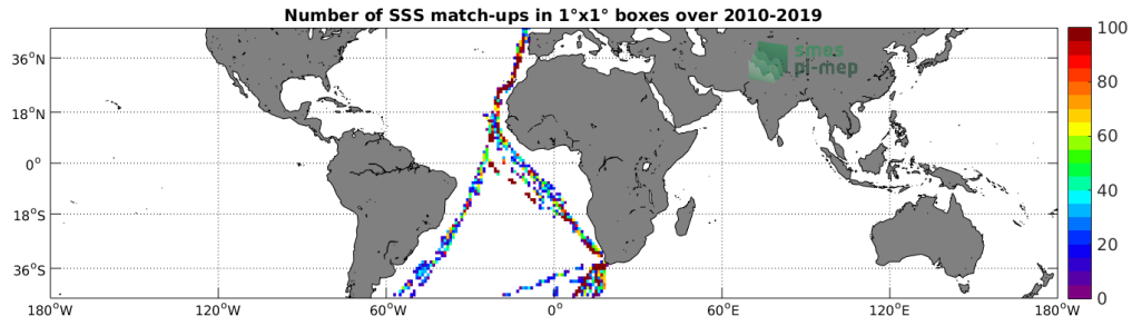
Figure 4: Number of SSS match-ups between TSG-POLARSTERN SSS and the SMOS L2 v662 (ESA) SSS product for the Mid-Low Latitudes 45N-45S Pi-MEP region over 1^\circ \times 1^\circ boxes and for the full satellite product period.
