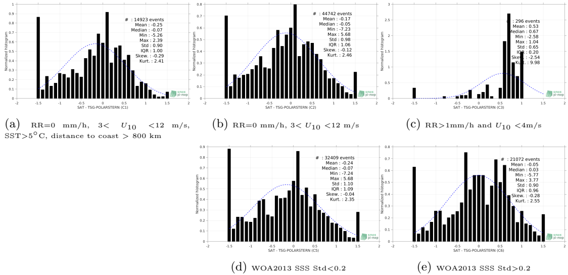
Figure 13: Normalized histogram of \Delta SSS (SMOS L2 v662 (ESA) - TSG-POLARSTERN) for 5 different subdatasets corresponding to: RR=0 mm/h, 3 < U_{10} < 12 m/s, SST > 5^\circ C , distance to coast > 800 km (a), RR=0 mm/h, 3 < U_{10} < 12 m/s (b), RR > 1 mm/h and U_{10} < 4 m/s (c), WOA2013 SSS Std < 0.2 (d), WOA2013 SSS Std > 0.2 (e).
