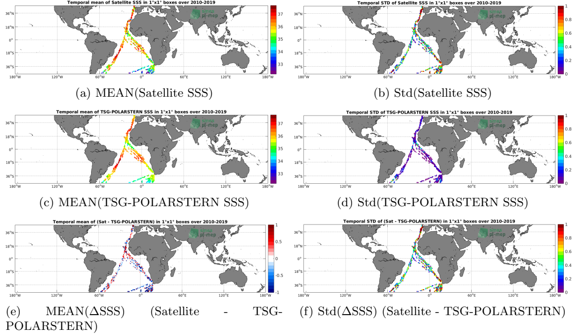
Figure 6: Temporal mean (left) and Std (right) of SSS from SMOS L2 v662 (ESA) (top), TSG-POLARSTERN (middle), and of \Delta SSS (Satellite - TSG-POLARSTERN). Only match-up pairs are used to generate these maps.
