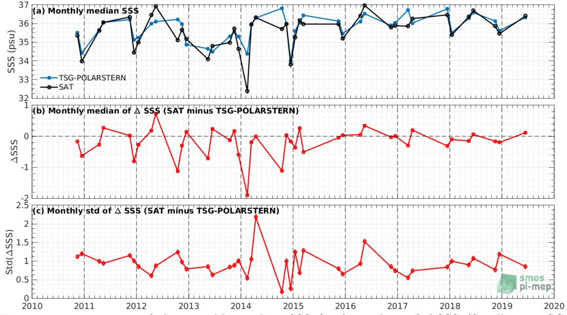
Figure 7: Time series of the monthly median SSS (top), median of \Delta\text{SSS} (Satellite - TSG-POLARSTERN) and Std of \Delta\text{SSS} (Satellite - TSG-POLARSTERN) over the Mid-Low Latitudes 45N-45S Pi-MEP region considering all match-ups collected by the Pi-MEP.
