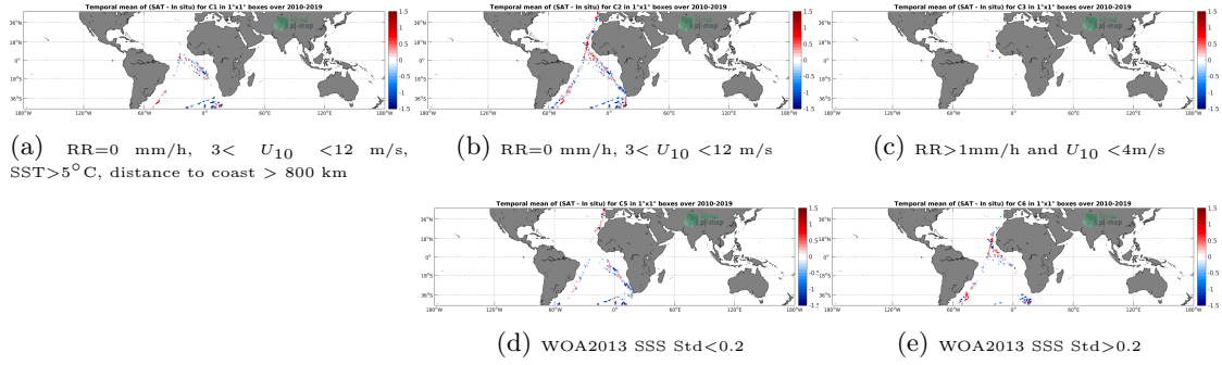
Figure 12: Temporal mean gridded over spatial boxes of size 1^\circ \times 1^\circ of \Delta SSS (SMOS L2 v662 (ESA) - TSG-POLARSTERN) for 5 different subdatasets corresponding to: RR=0 mm/h, 3 < U_{10} < 12 m/s, SST > 5^\circ C , distance to coast > 800 km (a), RR=0 mm/h, 3 < U_{10} < 12 m/s (b), RR > 1 mm/h and U_{10} < 4 m/s (c), WOA2013 SSS Std < 0.2 (d), WOA2013 SSS Std > 0.2 (e).
