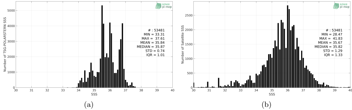
Figure 2: Histograms of SSS from TSG-POLARSTERN (a) and SMOS L2 v662 (ESA) (b) considering all match-up pairs per bins of 0.1 over the Mid-Low Latitudes 45N-45S Pi-MEP region and for the full satellite product period.
