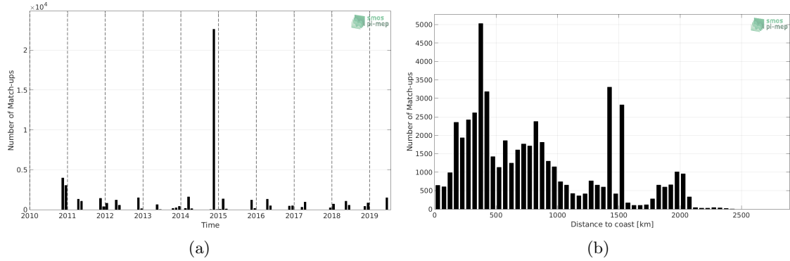
Figure 1: Number of match-ups between TSG-POLARSTERN and SMOS L2 v662 (ESA) SSS as a function of time (a) and as function of the distance to coast (b) over the Mid-Low Latitudes 45N-45S Pi-MEP region and for the full satellite product period.
