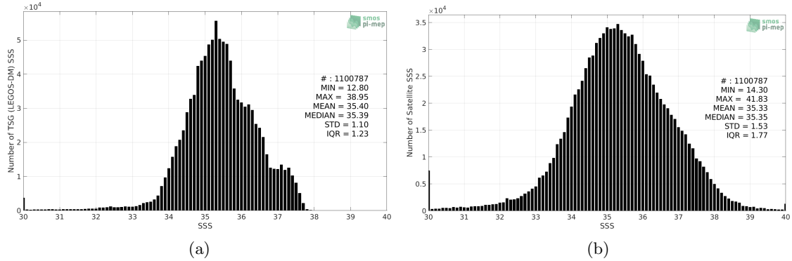
Figure 2: Histograms of SSS pairs from TSG (LEGOS-DM) (a) and SMOS SSS L2 v662 (ESA) (b) considering all match-up pairs per bins of 0.1 over the Mid-Low Latitudes 45N-45S Pi-MEP region and for the full satellite product period.
