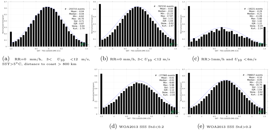
Figure 13: Normalized histogram of \Delta SSS (SMOS SSS L2 v662 (ESA) - TSG (LEGOS-DM)) for 5 different subdatasets corresponding to: RR=0 mm/h, 3 < U_{10} < 12 m/s, SST >5^\circ\text{C} , distance to coast > 800 km (a), RR=0 mm/h, 3 < U_{10} < 12 m/s (b), RR >1 mm/h and U_{10} < 4 m/s (c), WOA2013 SSS Std <0.2 (d), WOA2013 SSS Std >0.2 (e).
