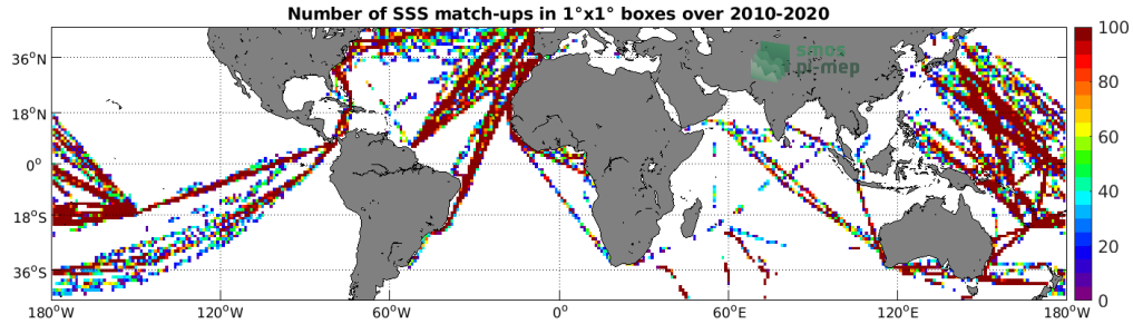
Figure 4: Number of SSS match-ups between TSG (LEGOS-DM) SSS and the SMOS SSS L2 v662 (ESA) SSS product for the Mid-Low Latitudes 45N-45S Pi-MEP region over 1^\circ \times 1^\circ boxes and for the full satellite product period.
