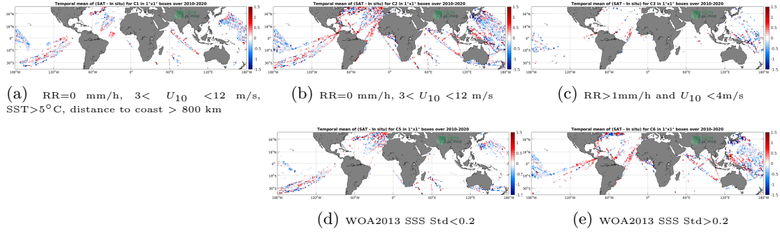
Figure 12: Temporal mean gridded over spatial boxes of size 1^\circ \times 1^\circ of \Delta SSS (SMOS SSS L2 v662 (ESA) - TSG (LEGOS-DM)) for 5 different subdatasets corresponding to: RR=0 mm/h, 3 < U_{10} < 12 m/s, SST >5^\circ\text{C} , distance to coast > 800 km (a), RR=0 mm/h, 3 < U_{10} < 12 m/s (b), RR >1 mm/h and U_{10} < 4 m/s (c), WOA2013 SSS Std <0.2 (d), WOA2013 SSS Std >0.2 (e).
