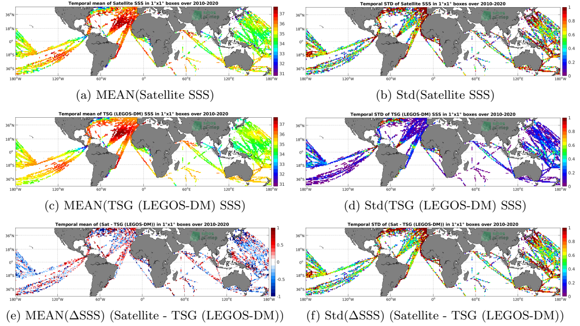
Figure 6: Temporal mean (left) and Std (right) of SSS from SMOS SSS L2 v662 (ESA) (top), TSG (LEGOS-DM) (middle), and of \Delta SSS (Satellite - TSG (LEGOS-DM)). Only match-up pairs are used to generate these maps.
