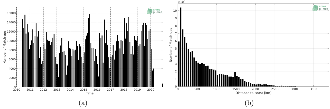
Figure 1: Number of match-ups between TSG (LEGOS-DM) and SMOS SSS L2 v662 (ESA) SSS as a function of time (a) and as function of the distance to coast (b) over the Mid-Low Latitudes 45N-45S Pi-MEP region and for the full satellite product period.
