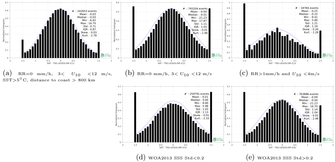
Figure 13: Normalized histogram of \Delta SSS (SMOS L2 v662 (ESA) - TSG-LEGOS-DM) for 5 different subdatasets corresponding to: RR=0 mm/h, 3 < U_{10} < 12 m/s, SST > 5^\circ C , distance to coast > 800 km (a), RR=0 mm/h, 3 < U_{10} < 12 m/s (b), RR > 1 mm/h and U_{10} < 4 m/s (c), WOA2013 SSS Std < 0.2 (d), WOA2013 SSS Std > 0.2 (e).
