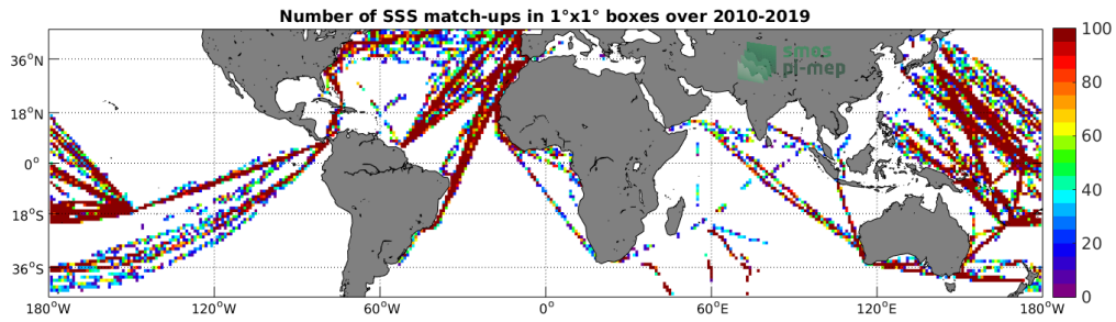
Figure 4: Number of SSS match-ups between TSG-LEGOS-DM SSS and the SMOS L2 v662 (ESA) SSS product for the Mid-Low Latitudes 45N-45S Pi-MEP region over 1°x1° boxes and for the full satellite product period.
