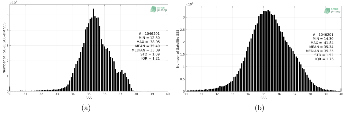
Figure 2: Histograms of SSS from TSG-LEGOS-DM (a) and SMOS L2 v662 (ESA) (b) considering all match-up pairs per bins of 0.1 over the Mid-Low Latitudes 45N-45S Pi-MEP region and for the full satellite product period.
