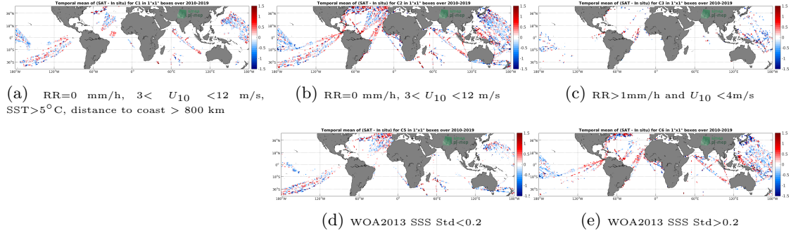
Figure 12: Temporal mean gridded over spatial boxes of size 1^\circ \times 1^\circ of \Delta SSS (SMOS L2 v662 (ESA) - TSG-LEGOS-DM) for 5 different subdatasets corresponding to: RR=0 mm/h, 3 < U_{10} < 12 m/s, SST > 5^\circ C , distance to coast > 800 km (a), RR=0 mm/h, 3 < U_{10} < 12 m/s (b), RR > 1 mm/h and U_{10} < 4 m/s (c), WOA2013 SSS Std < 0.2 (d), WOA2013 SSS Std > 0.2 (e).
