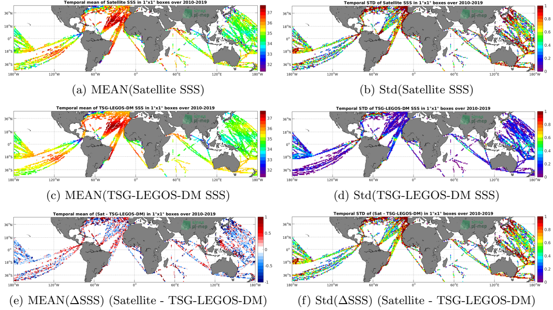
Figure 6: Temporal mean (left) and Std (right) of SSS from SMOS L2 v662 (ESA) (top), TSG-LEGOS-DM (middle), and of \Delta SSS (Satellite - TSG-LEGOS-DM). Only match-up pairs are used to generate these maps.
