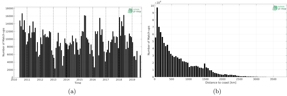
Figure 1: Number of match-ups between TSG-LEGOS-DM and SMOS L2 v662 (ESA) SSS as a function of time (a) and as function of the distance to coast (b) over the Mid-Low Latitudes 45N-45S Pi-MEP region and for the full satellite product period.
