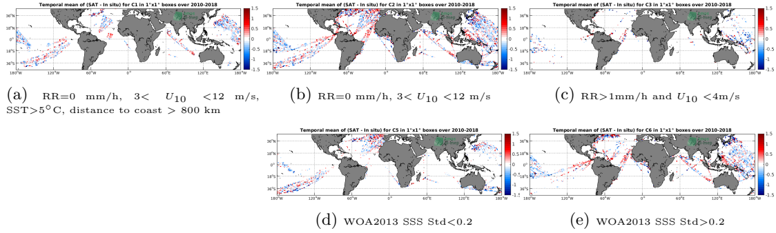
Figure 12: Temporal mean gridded over spatial boxes of size 1^\circ \times 1^\circ of \Delta SSS (SMOS-L2-DPGS-v662 - TSG-LEGOS-DM) for 5 different subdatasets corresponding to: RR=0 mm/h, 3 < U_{10} < 12 m/s, SST > 5^\circ C , distance to coast > 800 km (a), RR=0 mm/h, 3 < U_{10} < 12 m/s (b), RR > 1 mm/h and U_{10} < 4 m/s (c), WOA2013 SSS Std < 0.2 (d), WOA2013 SSS Std > 0.2 (e).
