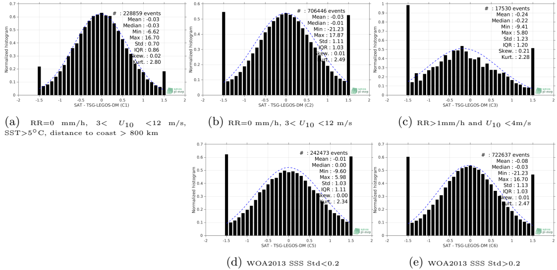
Figure 13: Normalized histogram of \Delta SSS (SMOS-L2-DPGS-v662 - TSG-LEGOS-DM) for 5 different subdatasets corresponding to: RR=0 mm/h, 3 < U_{10} < 12 m/s, SST > 5^\circ C , distance to coast > 800 km (a), RR=0 mm/h, 3 < U_{10} < 12 m/s (b), RR > 1 mm/h and U_{10} < 4 m/s (c), WOA2013 SSS Std < 0.2 (d), WOA2013 SSS Std > 0.2 (e).
