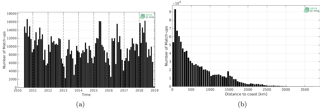
Figure 1: Number of match-ups between TSG-LEGOS-DM and SMOS-L2-DPGS-v662 SSS as a function of time (a) and as function of the distance to coast (b) over the Mid-Low Latitudes 45N-45S Pi-MEP region and for the full satellite product period.
