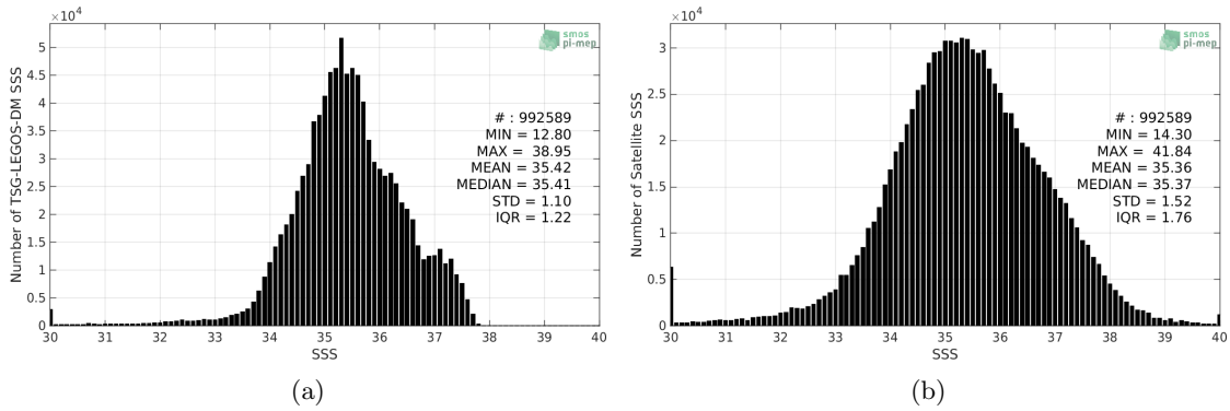
Figure 2: Histograms of SSS from TSG-LEGOS-DM (a) and SMOS-L2-DPGS-v662 (b) considering all match-up pairs per bins of 0.1 over the Mid-Low Latitudes 45N-45S Pi-MEP region and for the full satellite product period.
