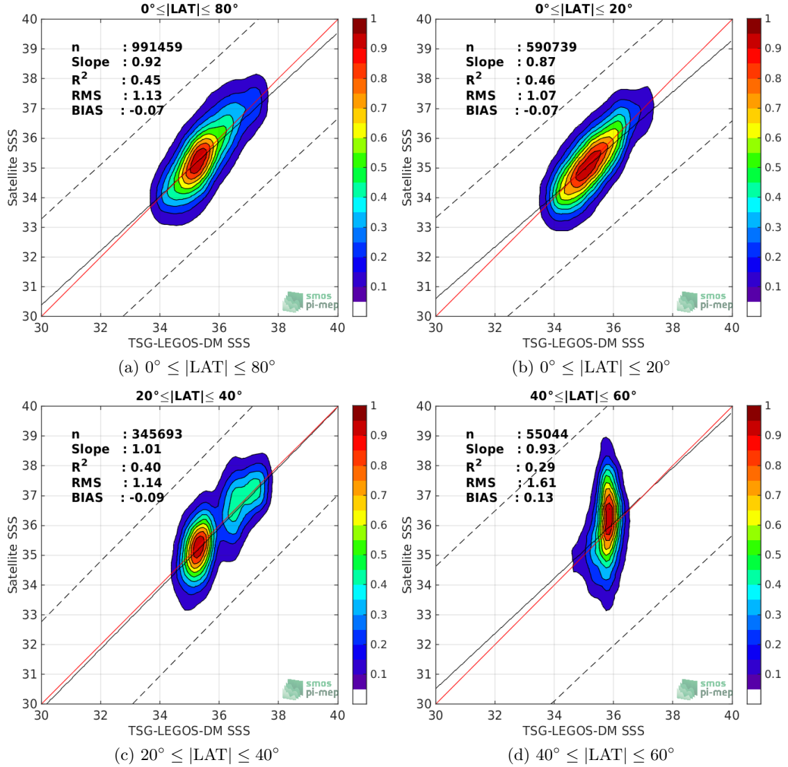
Figure 9: Contour maps of the concentration of SMOS-L2-DPGS-v662 SSS (y-axis) versus TSG-LEGOS-DM SSS (x-axis) at match-up pairs for different latitude bands. For each plot, the red line shows x=y . The black thin and dashed lines indicate a linear fit through the data cloud and the \pm 95\% confidence levels, respectively. The number match-up pairs n , the slope and R^2 coefficient of the linear fit, the root mean square (RMS) and the mean bias between satellite and in situ data are indicated for each latitude band in each plots.
