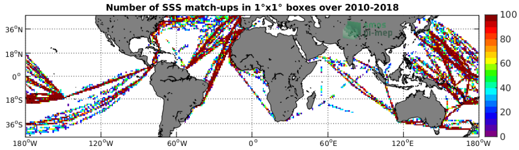
Figure 4: Number of SSS match-ups between TSG-LEGOS-DM SSS and the SMOS-L2-DPGS-v662 SSS product for the Mid-Low Latitudes 45N-45S Pi-MEP region over 1^\circ \times 1^\circ boxes and for the full satellite product period.
