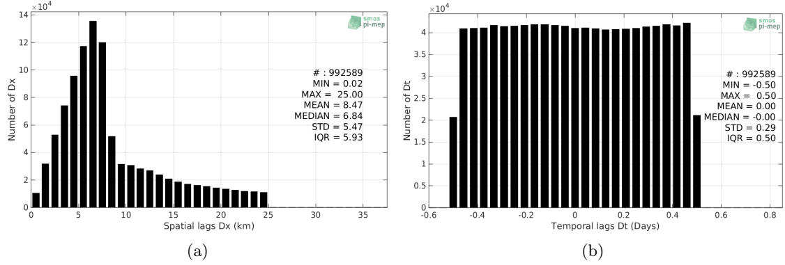
Figure 5: Histograms of the spatial (a) and temporal (b) lags between the time of the TSG-LEGOS-DM measurements and the date of the corresponding SMOS-L2-DPGS-v662 SSS product.
