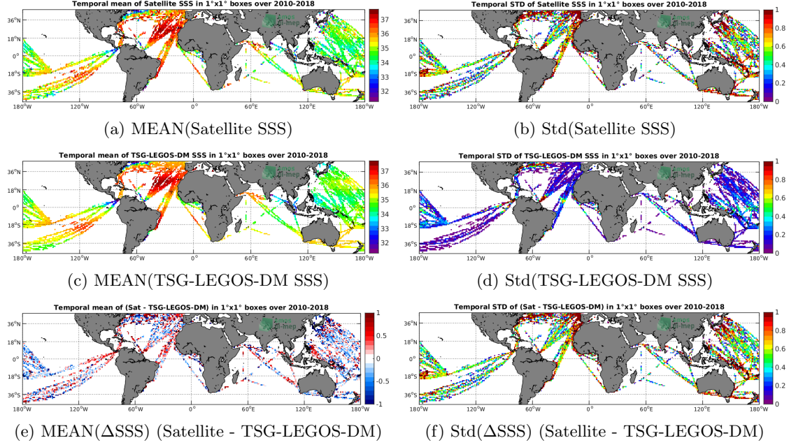
Figure 6: Temporal mean (left) and Std (right) of SSS from SMOS-L2-DPGS-v662 (top), TSG-LEGOS-DM (middle), and of \Delta SSS (Satellite - TSG-LEGOS-DM). Only match-up pairs are used to generate these maps.
