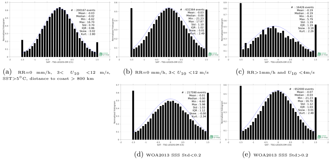
Figure 13: Normalized histogram of \Delta SSS (SMOS-L2-DPGS-v662 - TSG-LEGOS-DM) for 5 different subdatasets corresponding to: RR=0 mm/h, 3 < U_{10} < 12 m/s, SST > 5^\circ C , distance to coast > 800 km (a), RR=0 mm/h, 3 < U_{10} < 12 m/s (b), RR > 1 mm/h and U_{10} < 4 m/s (c), WOA2013 SSS Std < 0.2 (d), WOA2013 SSS Std > 0.2 (e).
