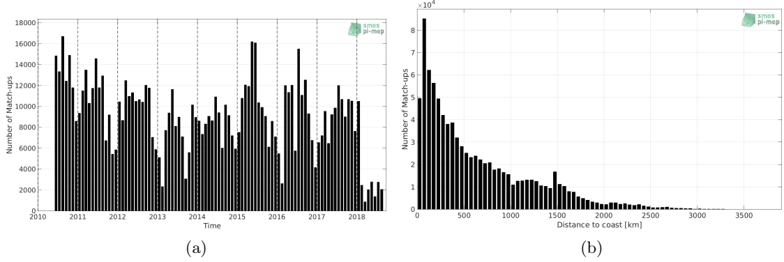
Figure 1: Number of match-ups between TSG-LEGOS-DM and SMOS-L2-DPGS-v662 SSS as a function of time (a) and as function of the distance to coast (b) over the Mid-Low Latitudes 45N-45S Pi-MEP region and for the full satellite product period.
