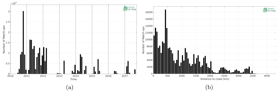
Figure 1: Number of match-ups between TSG-GOSUD-Sailing-ship and SMOS L2 v662 (ESA) SSS as a function of time (a) and as function of the distance to coast (b) over the Mid-Low Latitudes 45N-45S Pi-MEP region and for the full satellite product period.
