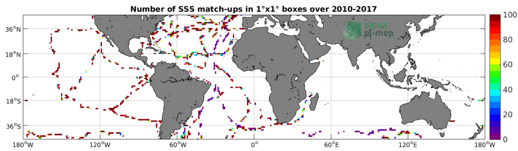
Figure 4: Number of SSS match-ups between TSG-GOSUD-Sailing-ship SSS and the SMOS L2 v662 (ESA) SSS product for the Mid-Low Latitudes 45N-45S Pi-MEP region over 1^\circ \times 1^\circ boxes and for the full satellite product period.
