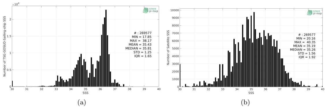
Figure 2: Histograms of SSS from TSG-GOSUD-Sailing-ship (a) and SMOS L2 v662 (ESA) (b) considering all match-up pairs per bins of 0.1 over the Mid-Low Latitudes 45N-45S Pi-MEP region and for the full satellite product period.
