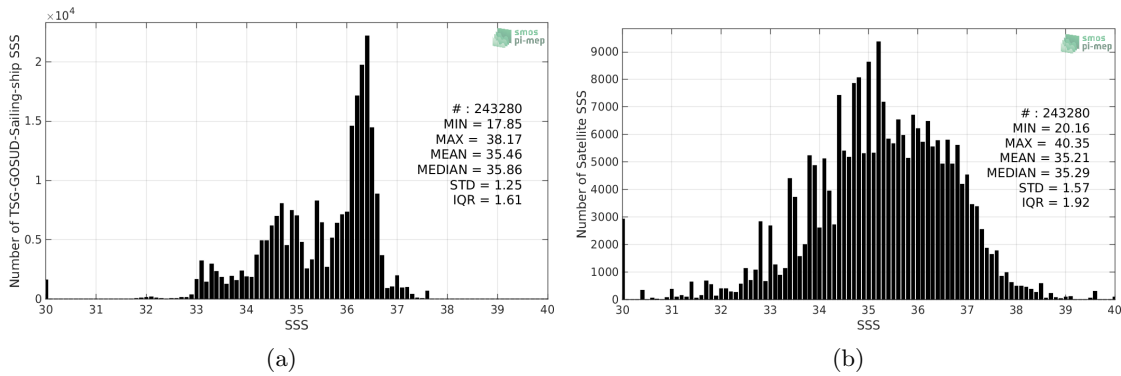
Figure 2: Histograms of SSS from TSG-GOSUD-Sailing-ship (a) and SMOS-L2-DPGS-v662 (b) considering all match-up pairs per bins of 0.1 over the Mid-Low Latitudes 45N-45S Pi-MEP region and for the full satellite product period.
