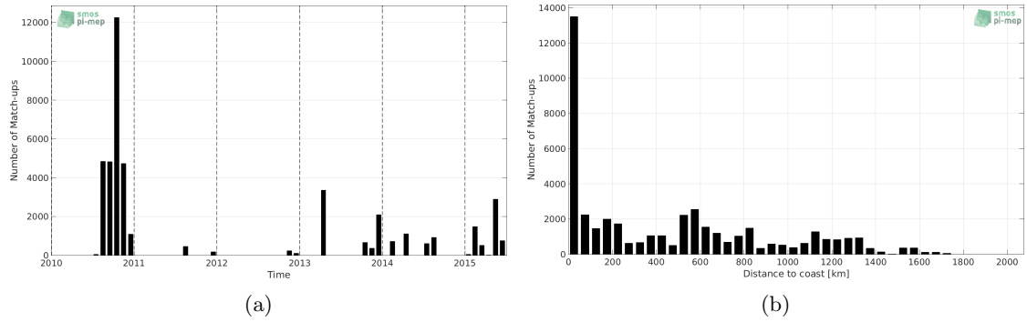
Figure 1: Number of match-ups between TSG-GOSUD-Sailing-ship and SMOS-L2-DPGS-v662 SSS as a function of time (a) and as function of the distance to coast (b) over the Mid-Low Latitudes 45N-45S Pi-MEP region and for the full satellite product period.
