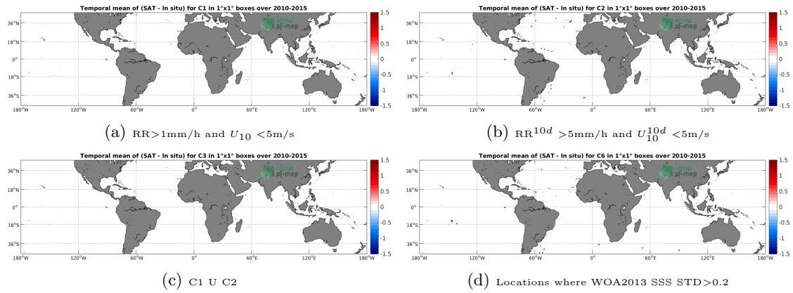
Figure 12: Temporal mean gridded over spatial boxes of size 1^\circ \times 1^\circ of \Delta SSS (SMOS-L2-DPGS-v662 - TSG-GOSUD-Sailing-ship) for 4 different subdatasets corresponding to: RR > 1\text{mm/h} and U_{10} < 5\text{m/s} (a), RR^{10d} > 5\text{mm/h} and U_{10}^{10d} < 5\text{m/s} (b), C1 U C2 (c), Locations where WOA2013 SSS STD > 0.2 (d).
