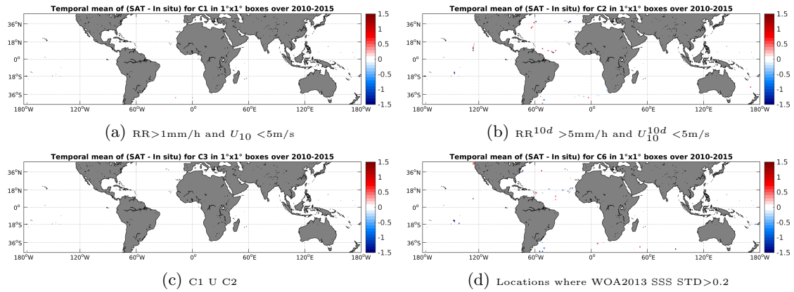
Figure 12: Temporal mean gridded over spatial boxes of size 1^\circ \times 1^\circ of \Delta SSS (SMOS-L2-DPGS-v662 - TSG-GOSUD-Sailing-ship) for 4 different subdatasets corresponding to:RR >1 mm/h and U_{10} < 5 m/s (a), RR 10d > 5 mm/h and U_{10}^{10d} < 5 m/s (b), C1 U C2 (c),Locations where WOA2013 SSS STD >0.2 (d).
