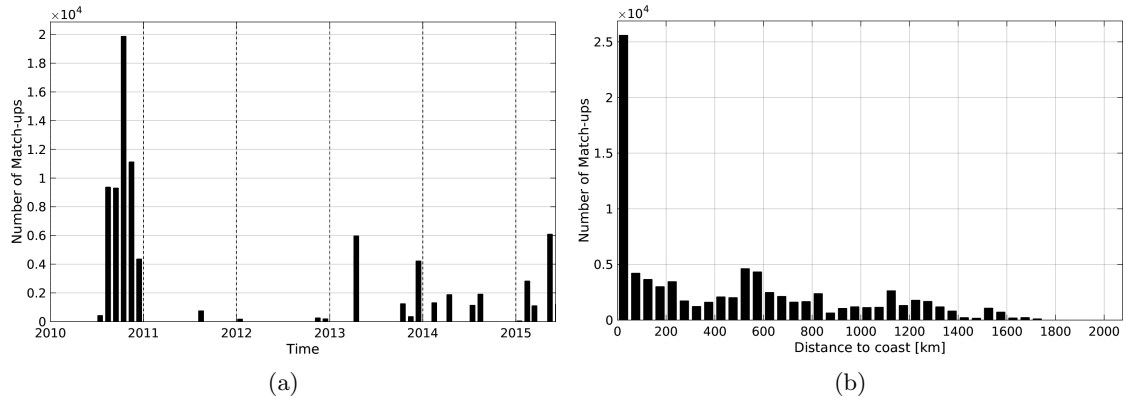
Figure 1: Number of match-ups between TSG-GOSUD-Sailing-ship and SMOS-L2-DPGS-v662 SSS as a function of time (a) and as function of the distance to coast (b) over the Mid-Low Latitudes 45N-45S Pi-MEP region and for the full satellite product period.
