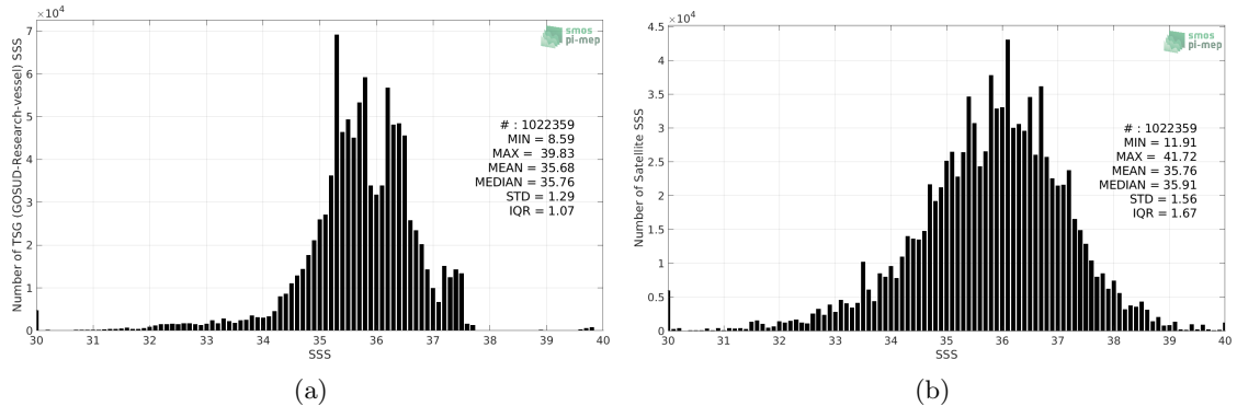
Figure 2: Histograms of SSS from TSG (GOSUD-Research-vessel) (a) and SMOS SSS L2 v662 (ESA) (b) considering all match-up pairs per bins of 0.1 over the Mid-Low Latitudes 45N-45S Pi-MEP region and for the full satellite product period.
