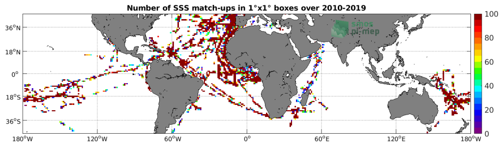
Figure 4: Number of SSS match-ups between TSG (GOSUD-Research-vessel) SSS and the SMOS SSS L2 v662 (ESA) SSS product for the Mid-Low Latitudes 45N-45S Pi-MEP region over 1^\circ \times 1^\circ boxes and for the full satellite product period.
