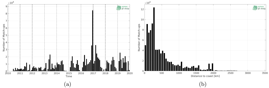
Figure 1: Number of match-ups between TSG (GOSUD-Research-vessel) and SMOS SSS L2 v662 (ESA) SSS as a function of time (a) and as function of the distance to coast (b) over the Mid-Low Latitudes 45N-45S Pi-MEP region and for the full satellite product period.
