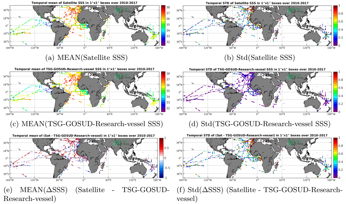
Figure 6: Temporal mean (left) and Std (right) of SSS from SMOS-L2-DPGS-v662 (top), TSG-GOSUD-Research-vessel (middle), and of \Delta SSS (Satellite - TSG-GOSUD-Research-vessel). Only match-up pairs are used to generate these maps.
