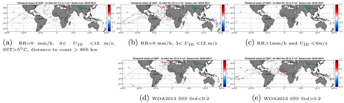
Figure 12: Temporal mean gridded over spatial boxes of size 1^\circ \times 1^\circ of \Delta SSS (SMOS-L2-DPGS-v662 - TSG-GOSUD-Research-vessel) for 5 different subdatasets corresponding to:RR=0 mm/h, 3 < U_{10} < 12 m/s, SST>5°C, distance to coast > 800 km (a), RR=0 mm/h, 3 < U_{10} < 12 m/s (b), RR>1mm/h and U_{10} < 4 m/s (c), WOA2013 SSS Std<0.2 (d), WOA2013 SSS Std>0.2 (e).
