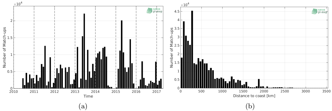
Figure 1: Number of match-ups between TSG-GOSUD-Research-vessel and SMOS-L2-DPGS-v662 SSS as a function of time (a) and as function of the distance to coast (b) over the Mid-Low Latitudes 45N-45S Pi-MEP region and for the full satellite product period.
