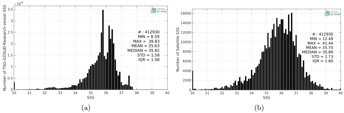
Figure 2: Histograms of SSS from TSG-GOSUD-Research-vessel (a) and SMOS-L2-DPGS-v662 (b) considering all match-up pairs per bins of 0.1 over the Mid-Low Latitudes 45N-45S Pi-MEP region and for the full satellite product period.
