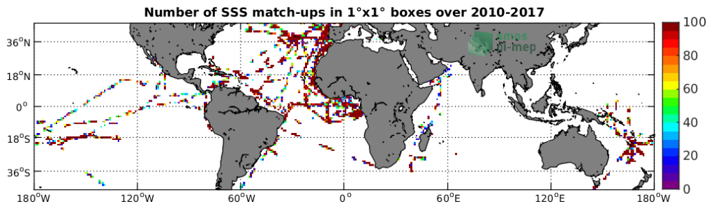
Figure 4: Number of SSS match-ups between TSG-GOSUD-Research-vessel SSS and the SMOS-L2-DPGS-v662 SSS product for the Mid-Low Latitudes 45N-45S Pi-MEP region over 1^\circ \times 1^\circ boxes and for the full satellite product period.
