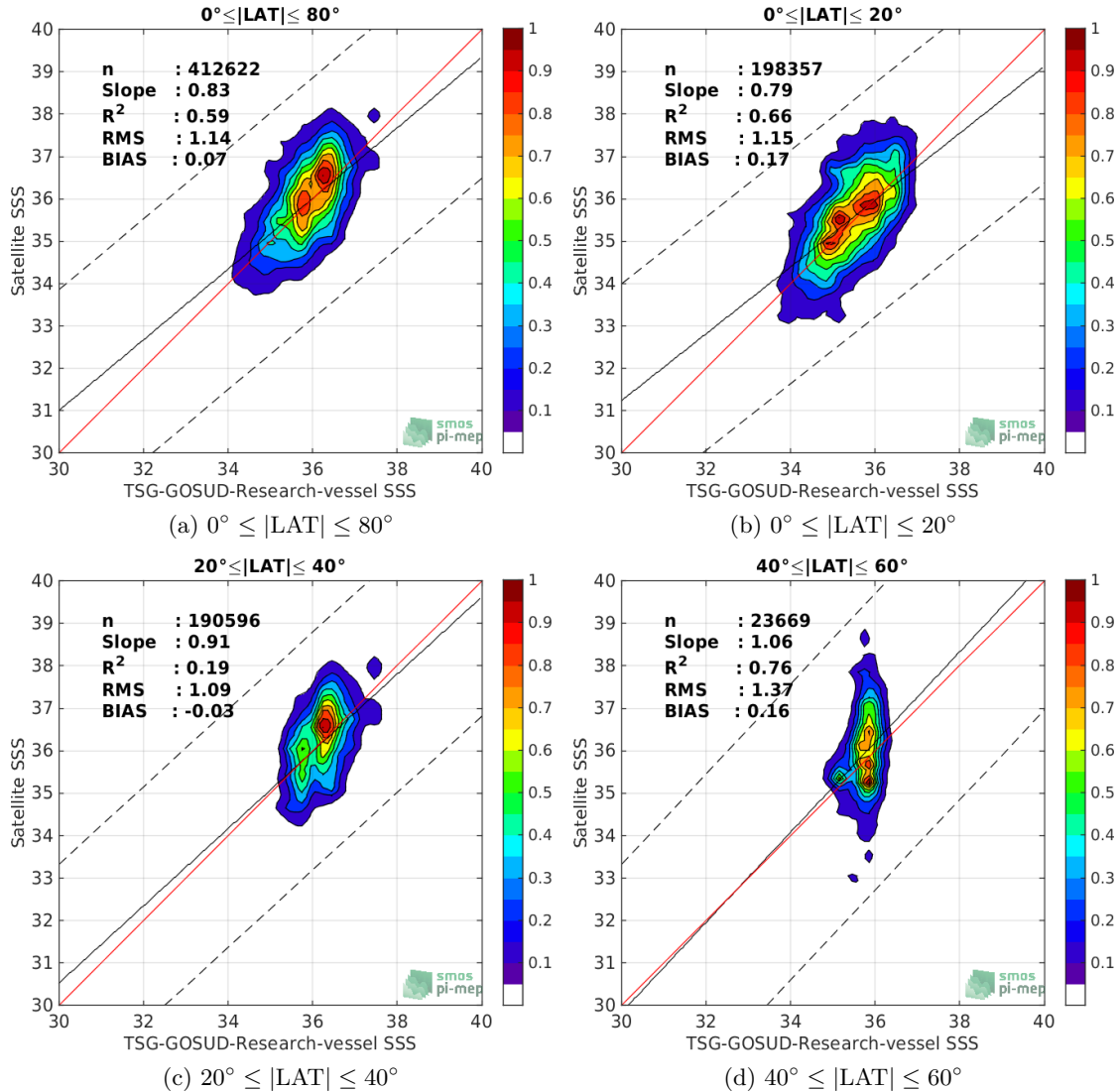
Figure 9: Contour maps of the concentration of SMOS-L2-DPGS-v662 SSS (y-axis) versus TSG-GOSUD-Research-vessel SSS (x-axis) at match-up pairs for different latitude bands. For each plot, the red line shows x=y . The black thin and dashed lines indicate a linear fit through the data cloud and the \pm 95\% confidence levels, respectively. The number match-up pairs n , the slope and R^2 coefficient of the linear fit, the root mean square (RMS) and the mean bias between satellite and in situ data are indicated for each latitude band in each plots.
