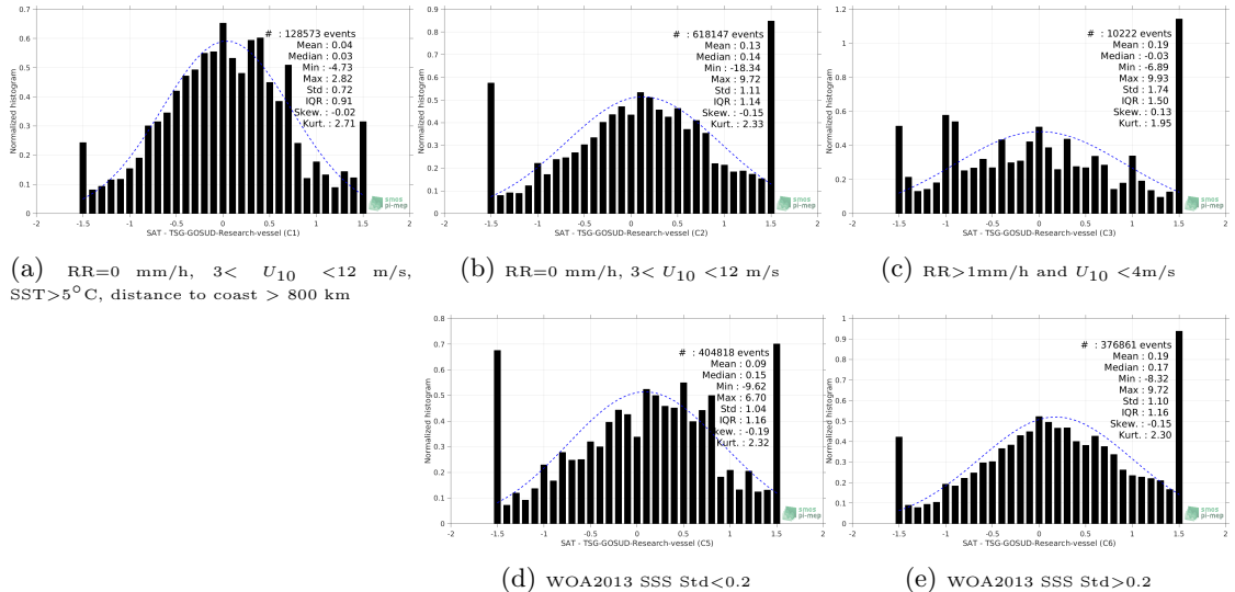
Figure 13: Normalized histogram of \Delta SSS (SMOS-L2-DPGS-v662 - TSG-GOSUD-Research-vessel) for 5 different subdatasets corresponding to: RR=0 mm/h, 3 < U_{10} < 12 m/s, SST >5^\circ\text{C} , distance to coast > 800 km (a), RR=0 mm/h, 3 < U_{10} < 12 m/s (b), RR >1 mm/h and U_{10} < 4 m/s (c), WOA2013 SSS Std <0.2 (d), WOA2013 SSS Std >0.2 (e).
