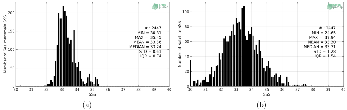
Figure 2: Histograms of SSS from Sea mammals (a) and SMOS-L2-DPGS-v662 (b) considering all match-up pairs per bins of 0.1 over the Mid-Low Latitudes 45N-45S Pi-MEP region and for the full satellite product period.
