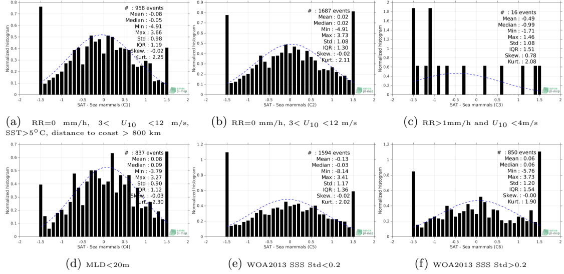
Figure 13: Normalized histogram of \Delta SSS (SMOS-L2-DPGS-v662 - Sea mammals) for 6 different subdatasets corresponding to: RR=0 mm/h, 3 < U_{10} < 12 m/s, SST > 5^\circ C , distance to coast > 800 km (a), RR=0 mm/h, 3 < U_{10} < 12 m/s (b), RR > 1 mm/h and U_{10} < 4 m/s (c), MLD < 20 m (d), WOA2013 SSS Std < 0.2 (e), WOA2013 SSS Std > 0.2 (f).
