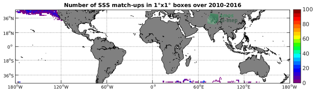
Figure 4: Number of SSS match-ups between Sea mammals SSS and the SMOS-L2-DPGS-v662 SSS product for the Mid-Low Latitudes 45N-45S Pi-MEP region over 1°x1° boxes and for the full satellite product period.
