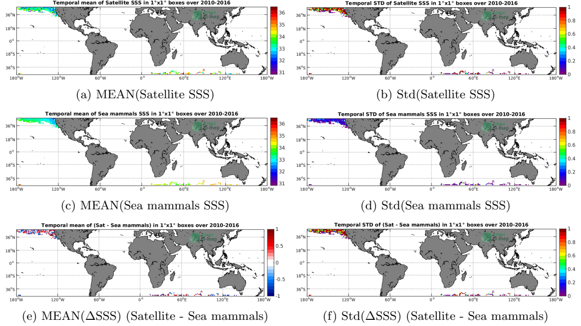
Figure 6: Temporal mean (left) and Std (right) of SSS from SMOS-L2-DPGS-v662 (top), Sea mammals (middle), and of \Delta SSS (Satellite - Sea mammals). Only match-up pairs are used to generate these maps.
