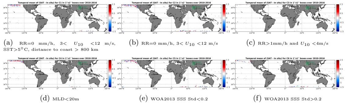
Figure 12: Temporal mean gridded over spatial boxes of size 1^\circ \times 1^\circ of \Delta SSS (SMOS-L2-DPGS-v662 - Sea mammals) for 6 different subdatasets corresponding to: RR=0 mm/h, 3 < U_{10} < 12 m/s, SST > 5^\circ C , distance to coast > 800 km (a), RR=0 mm/h, 3 < U_{10} < 12 m/s (b), RR > 1 mm/h and U_{10} < 4 m/s (c), MLD < 20 m (d), WOA2013 SSS Std < 0.2 (e), WOA2013 SSS Std > 0.2 (f).
