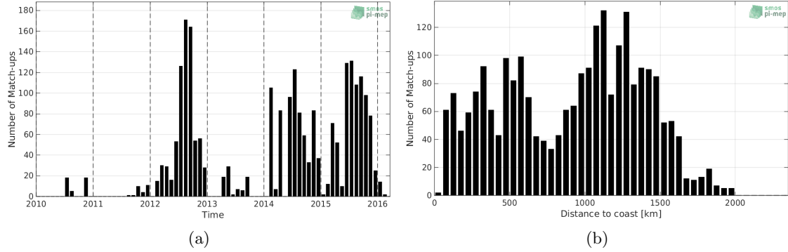
Figure 1: Number of match-ups between Sea mammals and SMOS-L2-DPGS-v662 SSS as a function of time (a) and as function of the distance to coast (b) over the Mid-Low Latitudes 45N-45S Pi-MEP region and for the full satellite product period.
