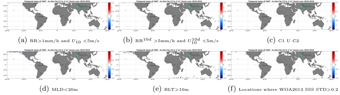
Figure 12: Temporal mean gridded over spatial boxes of size 1^\circ \times 1^\circ of \Delta\text{SSS} (SMOS-L2-DPGS-v662 - Sea mammals) for 6 different subdatasets corresponding to: \text{RR}>1\text{mm/h} and U_{10}<5\text{m/s} (a), \text{RR}^{10d}>5\text{mm/h} and U_{10}^{10d}<5\text{m/s} (b), C1 U C2 (c), \text{MLD}<20\text{m} (d), \text{BLT}>10\text{m} (e), Locations where WOA2013 SSS STD >0.2 (f).
