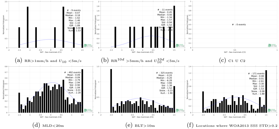
Figure 13: Normalized histogram of \Delta\text{SSS} (SMOS-L2-DPGS-v662 - Sea mammals) for 6 different subdatasets corresponding to: \text{RR}>1\text{mm/h} and U_{10}<5\text{m/s} (a), \text{RR}^{10d}>5\text{mm/h} and U_{10}^{10d}<5\text{m/s} (b), C1 U C2 (c), \text{MLD}<20\text{m} (d), \text{BLT}>10\text{m} (e), Locations where WOA2013 SSS STD >0.2 (f).
