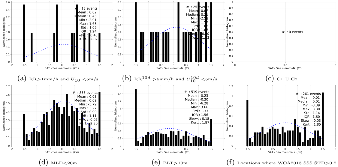
Figure 13: Normalized histogram of \Delta SSS (SMOS-L2-DPGS-v662 - Sea mammals) for 6 different subdatasets corresponding to: RR > 1\text{mm/h} and U_{10} < 5\text{m/s} (a), RR^{10d} > 5\text{mm/h} and U_{10}^{10d} < 5\text{m/s} (b), C1 U C2 (c), MLD < 20\text{m} (d), BLT > 10\text{m} (e), Locations where WOA2013 SSS STD > 0.2 (f).
