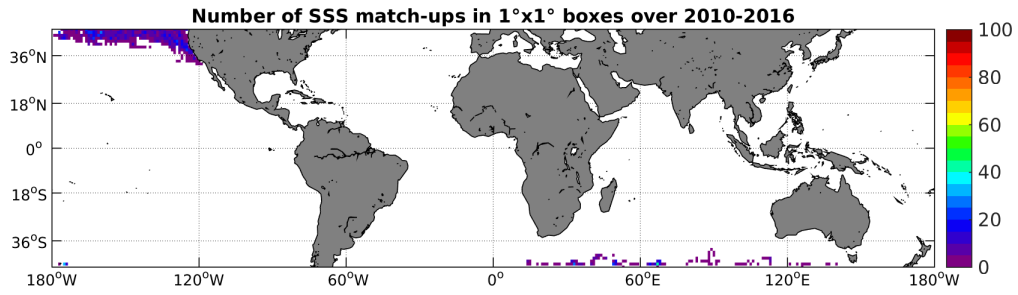
Figure 4: Number of SSS match-ups between Sea mammals SSS and the SMOS-L2-DPGS-v662 SSS product for the Mid-Low Latitudes 45N-45S Pi-MEP region over 1^\circ \times 1^\circ boxes and for the full satellite product period.
