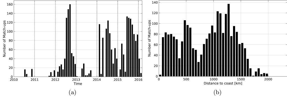
Figure 1: Number of match-ups between Sea mammals and SMOS-L2-DPGS-v662 SSS as a function of time (a) and as function of the distance to coast (b) over the Mid-Low Latitudes 45N-45S Pi-MEP region and for the full satellite product period.
