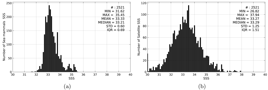
Figure 2: Histograms of SSS from Sea mammals (a) and SMOS-L2-DPGS-v662 (b) considering all match-up pairs per bins of 0.1 over the Mid-Low Latitudes 45N-45S Pi-MEP region and for the full satellite product period.
