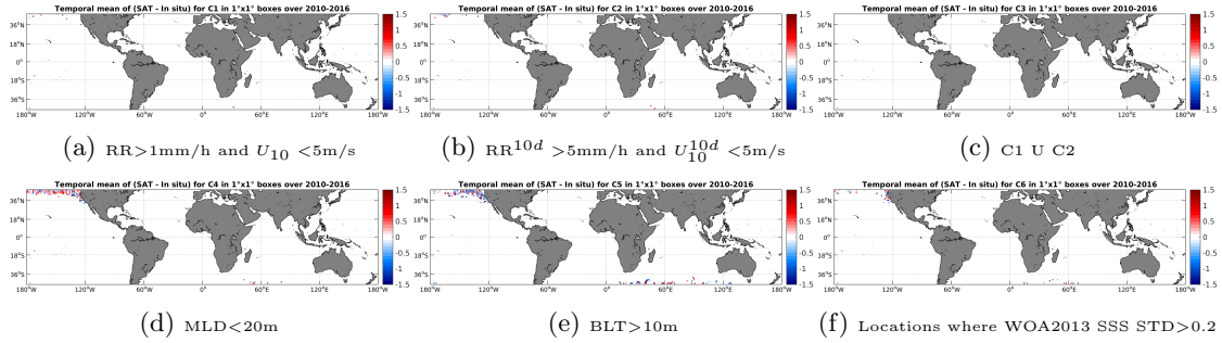
Figure 12: Temporal mean gridded over spatial boxes of size 1^\circ \times 1^\circ of \Delta SSS (SMOS-L2-DPGS-v662 - Sea mammals) for 6 different subdatasets corresponding to: RR > 1\text{mm/h} and U_{10} < 5\text{m/s} (a), RR^{10d} > 5\text{mm/h} and U_{10}^{10d} < 5\text{m/s} (b), C1 U C2 (c), MLD < 20\text{m} (d), BLT > 10\text{m} (e), Locations where WOA2013 SSS STD > 0.2 (f).
