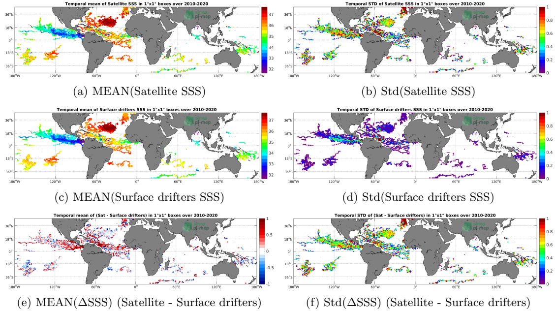
Figure 5: Temporal mean (left) and Std (right) of SSS from SMOS SSS L2 v662 (ESA) (top), Surface drifters (middle), and of \Delta\text{SSS} (Satellite - Surface drifters). Only match-up pairs are used to generate these maps.
