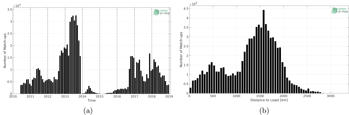
Figure 1: Number of match-ups between Surface drifters and SMOS L2 v662 (ESA) SSS as a function of time (a) and as function of the distance to coast (b) over the Mid-Low Latitudes 45N-45S Pi-MEP region and for the full satellite product period.
