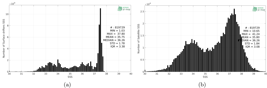
Figure 2: Histograms of SSS from Surface drifters (a) and SMOS L2 v662 (ESA) (b) considering all match-up pairs per bins of 0.1 over the Mid-Low Latitudes 45N-45S Pi-MEP region and for the full satellite product period.
