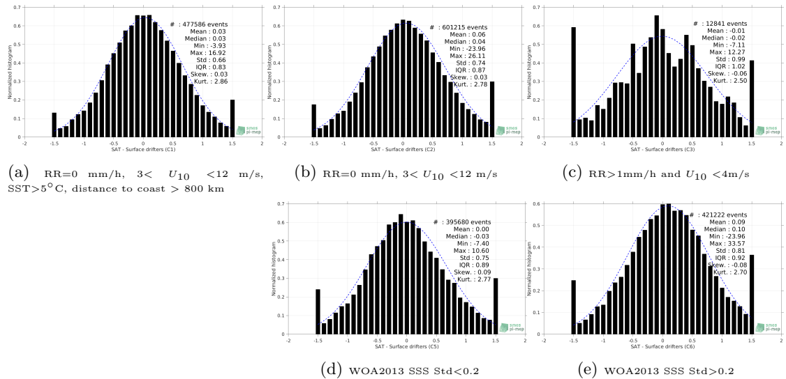
Figure 12: Normalized histogram of \Delta SSS (SMOS L2 v662 (ESA) - Surface drifters) for 5 different subdatasets corresponding to: RR=0 mm/h, 3 < U_{10} < 12 m/s, SST >5^\circ\text{C} , distance to coast > 800 km (a), RR=0 mm/h, 3 < U_{10} < 12 m/s (b), RR >1 mm/h and U_{10} < 4 m/s (c), WOA2013 SSS Std <0.2 (d), WOA2013 SSS Std >0.2 (e).
