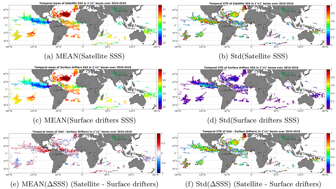
Figure 5: Temporal mean (left) and Std (right) of SSS from SMOS L2 v662 (ESA) (top), Surface drifters (middle), and of \Delta SSS (Satellite - Surface drifters). Only match-up pairs are used to generate these maps.
