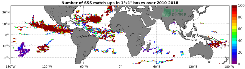
Figure 3: Number of SSS match-ups between Surface drifters SSS and the SMOS L2 v662 (ESA) SSS product for the Mid-Low Latitudes 45N-45S Pi-MEP region over 1^\circ \times 1^\circ boxes and for the full satellite product period.
