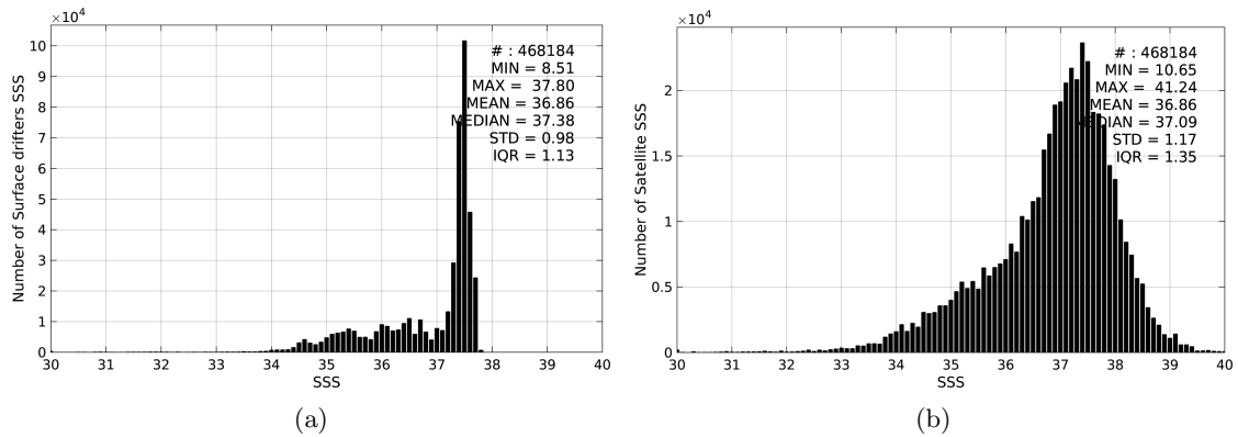
Figure 2: Histograms of SSS from Surface drifters (a) and SMOS-L2-DPGS-v662 (b) considering all match-up pairs per bins of 0.1 over the Mid-Low Latitudes 45N-45S Pi-MEP region and for the full satellite product period.
