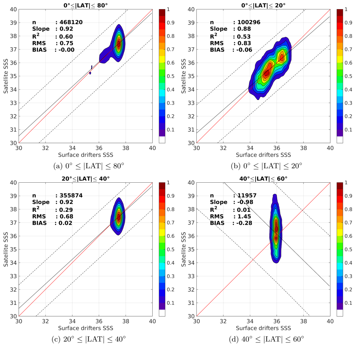
Figure 8: Contour maps of the concentration of SMOS-L2-DPGS-v662 SSS (y-axis) versus Surface drifters SSS (x-axis) at match-up pairs for different latitude bands. For each plot, the red line shows x=y . The black thin and dashed lines indicate a linear fit through the data cloud and the \pm 95\% confidence levels, respectively. The number match-up pairs n , the slope and R^2 coefficient of the linear fit, the root mean square (RMS) and the mean bias between satellite and in situ data are indicated for each latitude band in each plots.
