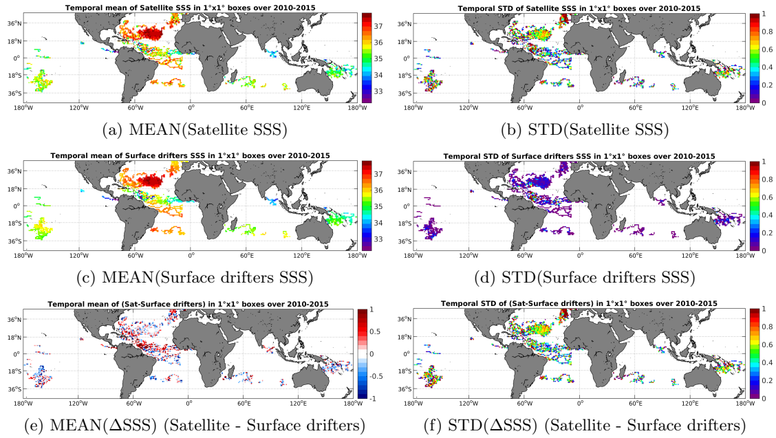
Figure 5: Temporal mean (left) and STD (right) of SSS from SMOS-L2-DPGS-v662 (top), Surface drifters (middle), and of \Delta SSS (Satellite - Surface drifters). Only match-up pairs are used to generate these maps.
