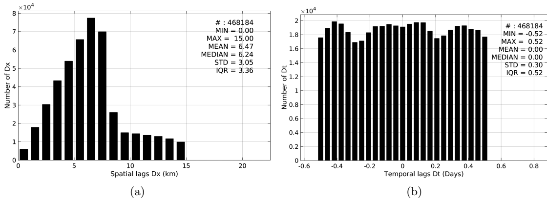
Figure 4: Histograms of the spatial (a) and temporal (b) lags between the time of the Surface drifters measurements and the date of the corresponding SMOS-L2-DPGS-v662 SSS product.
