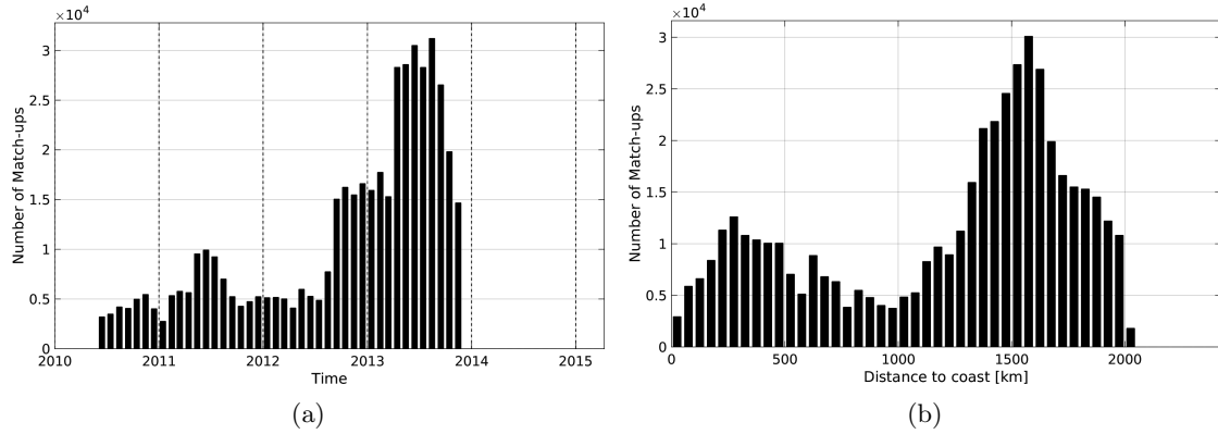
Figure 1: Number of match-ups between Surface drifters and SMOS-L2-DPGS-v662 SSS as a function of time (a) and as function of the distance to coast (b) over the Mid-Low Latitudes 45N-45S Pi-MEP region and for the full satellite product period.
