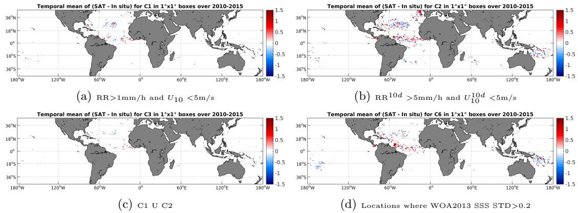
Figure 11: Temporal mean gridded over spatial boxes of size 1^\circ \times 1^\circ of \Delta SSS (SMOS-L2-DPGS-v662 - Surface drifters) for 4 different subdatasets corresponding to: RR > 1\text{mm/h} and U_{10} < 5\text{m/s} (a), RR^{10d} > 5\text{mm/h} and U_{10}^{10d} < 5\text{m/s} (b), C1 U C2 (c), Locations where WOA2013 SSS STD > 0.2 (d).
