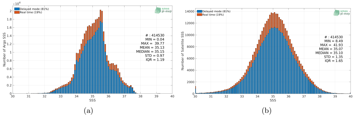
Figure 2: Histograms of SSS from Argo (a) and SMOS SSS L2 v662 (ESA) (b) considering all match-up pairs per bins of 0.1 over the Mid-Low Latitudes 45N-45S Pi-MEP region and for the full satellite product period.
