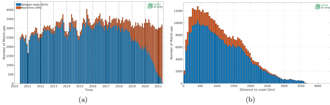
Figure 1: Number of match-ups between Argo and SMOS SSS L2 v662 (ESA) SSS as a function of time (a) and as function of the distance to coast (b) over the Mid-Low Latitudes 45N-45S Pi-MEP region and for the full satellite product period.
