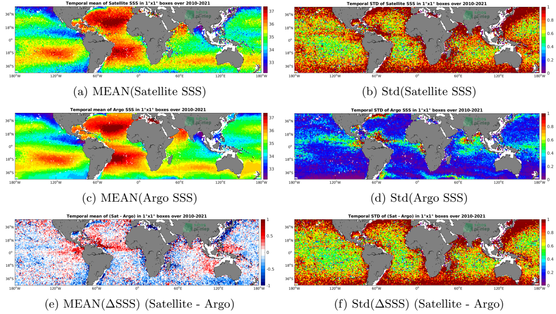
Figure 6: Temporal mean (left) and Std (right) of SSS from SMOS SSS L2 v662 (ESA) (top), Argo (middle), and of \Delta SSS (Satellite - Argo). Only match-up pairs are used to generate these maps.
