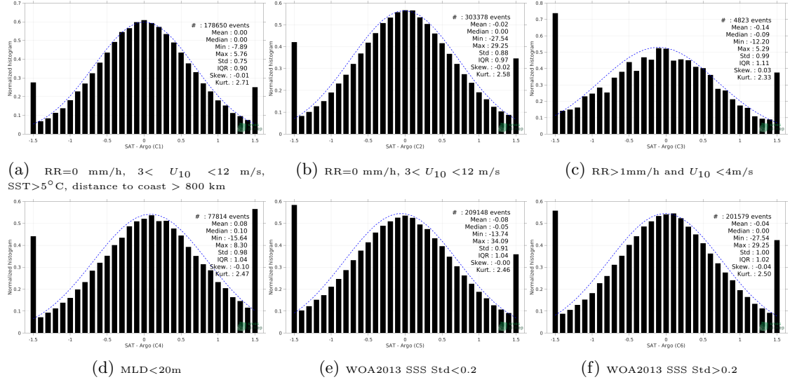
Figure 13: Normalized histogram of \Delta\text{SSS} (SMOS SSS L2 v662 (ESA) - Argo) for 6 different subdatasets corresponding to: RR=0 mm/h, 3 < U_{10} < 12 m/s, SST>5°C, distance to coast > 800 km (a), RR=0 mm/h, 3 < U_{10} < 12 m/s (b), RR>1mm/h and U_{10} < 4 m/s (c), MLD<20m (d), WOA2013 SSS Std<0.2 (e), WOA2013 SSS Std>0.2 (f).
