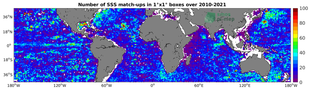
Figure 4: Number of SSS match-ups between Argo SSS and the SMOS SSS L2 v662 (ESA) SSS product for the Mid-Low Latitudes 45N-45S Pi-MEP region over 1^\circ \times 1^\circ boxes and for the full satellite product period.
