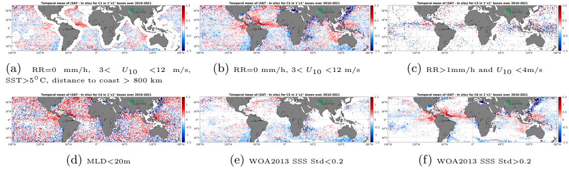
Figure 12: Temporal mean gridded over spatial boxes of size 1^\circ \times 1^\circ of \Delta SSS (SMOS SSS L2 v662 (ESA) - Argo) for 6 different subdatasets corresponding to: RR=0 mm/h, 3 < U_{10} < 12 m/s, SST > 5^\circ C , distance to coast > 800 km (a), RR=0 mm/h, 3 < U_{10} < 12 m/s (b), RR > 1 mm/h and U_{10} < 4 m/s (c), MLD < 20 m (d), WOA2013 SSS Std < 0.2 (e), WOA2013 SSS Std > 0.2 (f).
