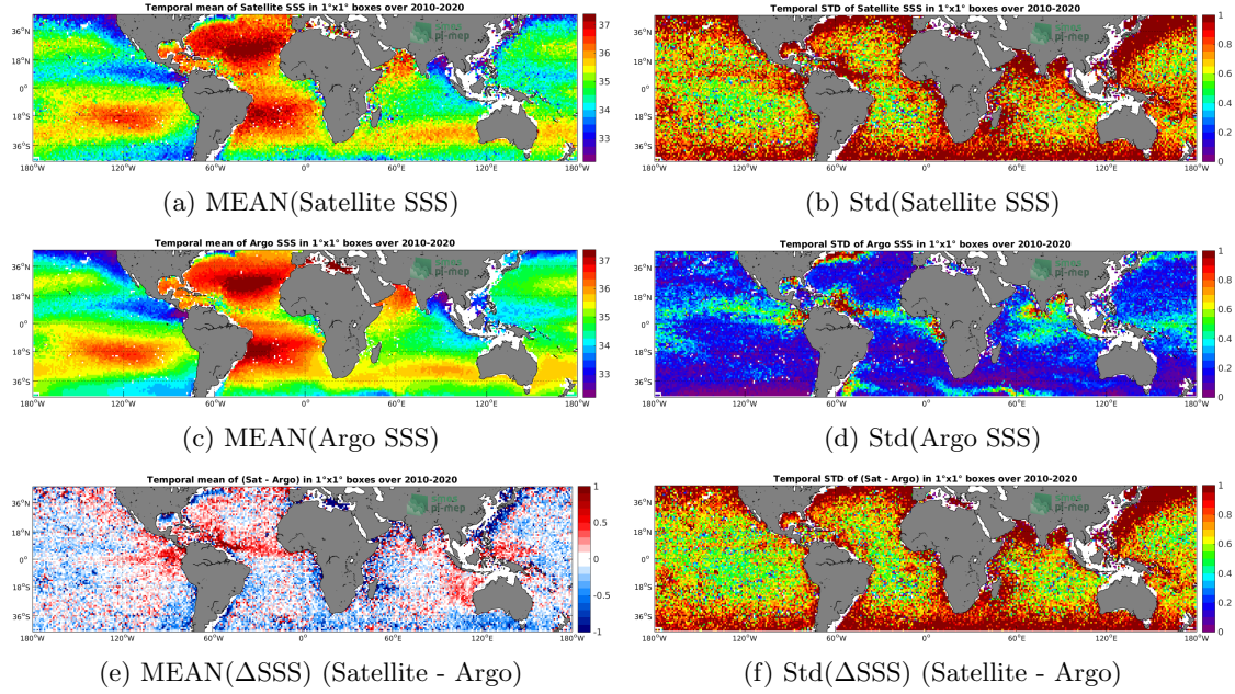
Figure 6: Temporal mean (left) and Std (right) of SSS from SMOS SSS L2 v662 (ESA) (top), Argo (middle), and of \Delta SSS (Satellite - Argo). Only match-up pairs are used to generate these maps.
