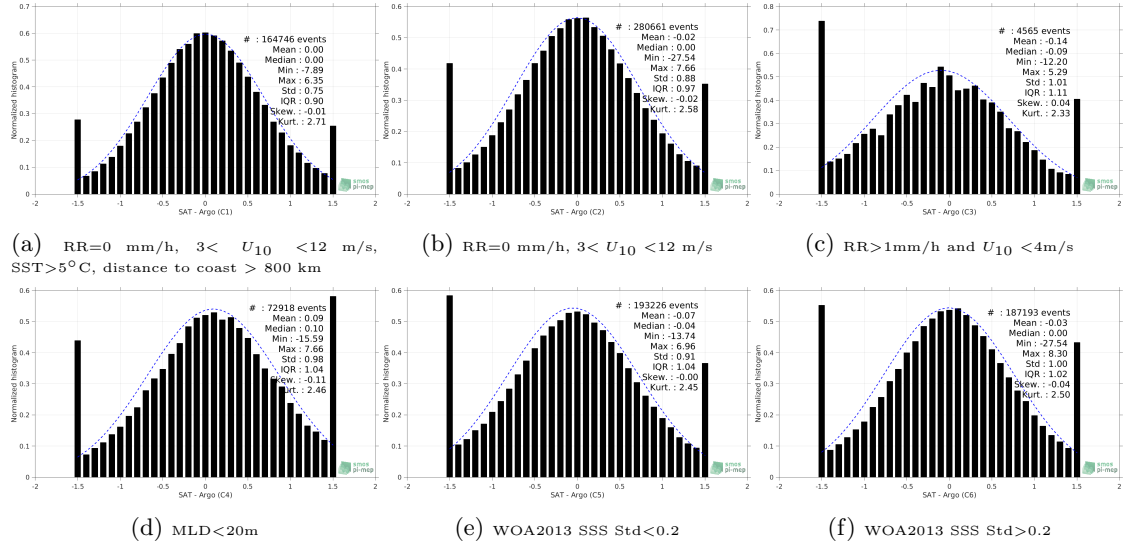
Figure 13: Normalized histogram of \Delta SSS (SMOS L2 v662 (ESA) - Argo) for 6 different subdatasets corresponding to: RR=0 mm/h, 3 < U_{10} < 12 m/s, SST >5^\circ\text{C} , distance to coast > 800 km (a), RR=0 mm/h, 3 < U_{10} < 12 m/s (b), RR >1 mm/h and U_{10} < 4 m/s (c), MLD <20 m (d), WOA2013 SSS Std <0.2 (e), WOA2013 SSS Std >0.2 (f).
