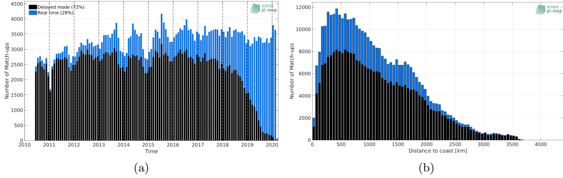
Figure 1: Number of match-ups between Argo and SMOS L2 v662 (ESA) SSS as a function of time (a) and as function of the distance to coast (b) over the Mid-Low Latitudes 45N-45S Pi-MEP region and for the full satellite product period.
