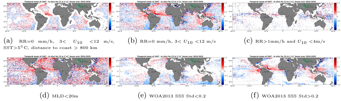
Figure 12: Temporal mean gridded over spatial boxes of size 1^\circ \times 1^\circ of \Delta SSS (SMOS L2 v662 (ESA) - Argo) for 6 different subdatasets corresponding to:RR=0 mm/h, 3 < U_{10} < 12 m/s, SST >5^\circ\text{C} , distance to coast > 800 km (a), RR=0 mm/h, 3 < U_{10} < 12 m/s (b), RR >1 mm/h and U_{10} < 4 m/s (c),MLD <20 m (d),WOA2013 SSS Std <0.2 (e),WOA2013 SSS Std >0.2 (f).
