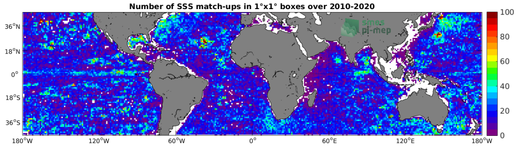
Figure 4: Number of SSS match-ups between Argo SSS and the SMOS L2 v662 (ESA) SSS product for the Mid-Low Latitudes 45N-45S Pi-MEP region over 1^\circ \times 1^\circ boxes and for the full satellite product period.
