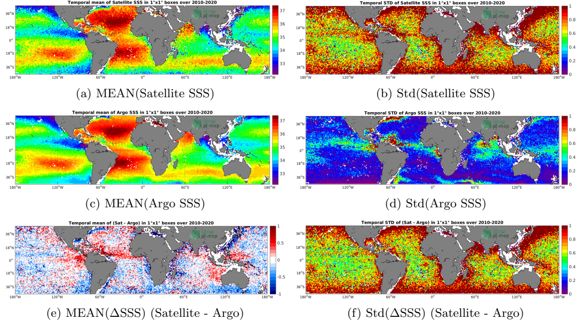
Figure 6: Temporal mean (left) and Std (right) of SSS from SMOS L2 v662 (ESA) (top), Argo (middle), and of \Delta SSS (Satellite - Argo). Only match-up pairs are used to generate these maps.
