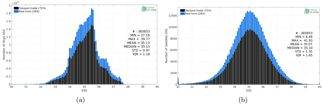
Figure 2: Histograms of SSS from Argo (a) and SMOS L2 v662 (ESA) (b) considering all match-up pairs per bins of 0.1 over the Mid-Low Latitudes 45N-45S Pi-MEP region and for the full satellite product period.
