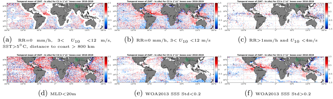
Figure 12: Temporal mean gridded over spatial boxes of size 1^\circ \times 1^\circ of \Delta SSS (SMOS-L2-DPGS-v662 - Argo) for 6 different subdatasets corresponding to:RR=0 mm/h, 3 < U_{10} < 12 m/s, SST >5^\circ C, distance to coast > 800 km (a), RR=0 mm/h, 3 < U_{10} < 12 m/s (b), RR >1 mm/h and U_{10} < 4 m/s (c),MLD <20 m (d),WOA2013 SSS Std <0.2 (e),WOA2013 SSS Std >0.2 (f).
