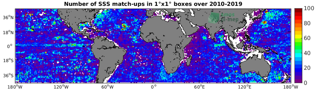
Figure 4: Number of SSS match-ups between Argo SSS and the SMOS-L2-DPGS-v662 SSS product for the Mid-Low Latitudes 45N-45S Pi-MEP region over 1^\circ \times 1^\circ boxes and for the full satellite product period.
