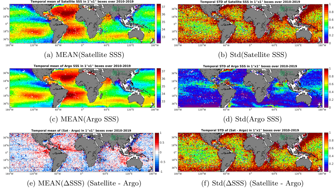
Figure 6: Temporal mean (left) and Std (right) of SSS from SMOS-L2-DPGS-v662 (top), Argo (middle), and of \Delta SSS (Satellite - Argo). Only match-up pairs are used to generate these maps.
