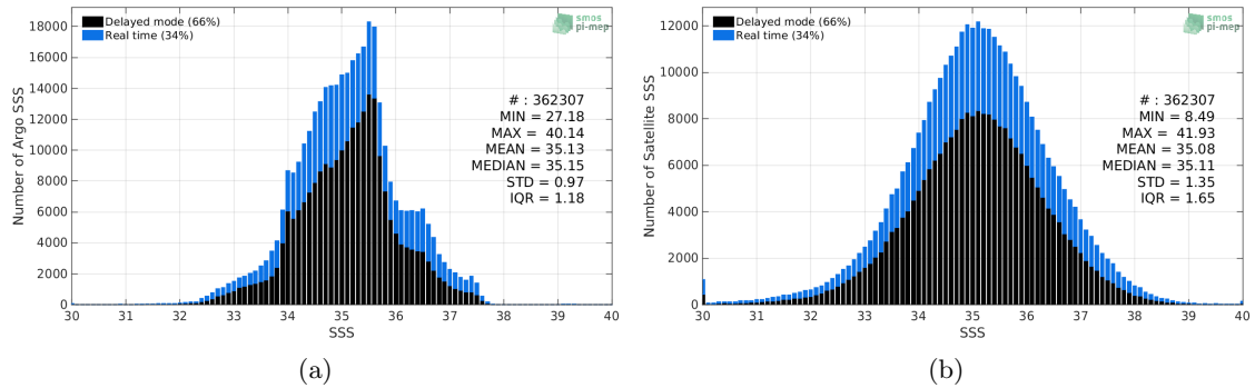
Figure 2: Histograms of SSS from Argo (a) and SMOS-L2-DPGS-v662 (b) considering all match-up pairs per bins of 0.1 over the Mid-Low Latitudes 45N-45S Pi-MEP region and for the full satellite product period.
