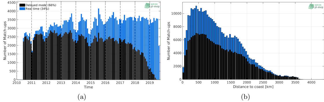
Figure 1: Number of match-ups between Argo and SMOS-L2-DPGS-v662 SSS as a function of time (a) and as function of the distance to coast (b) over the Mid-Low Latitudes 45N-45S Pi-MEP region and for the full satellite product period.
