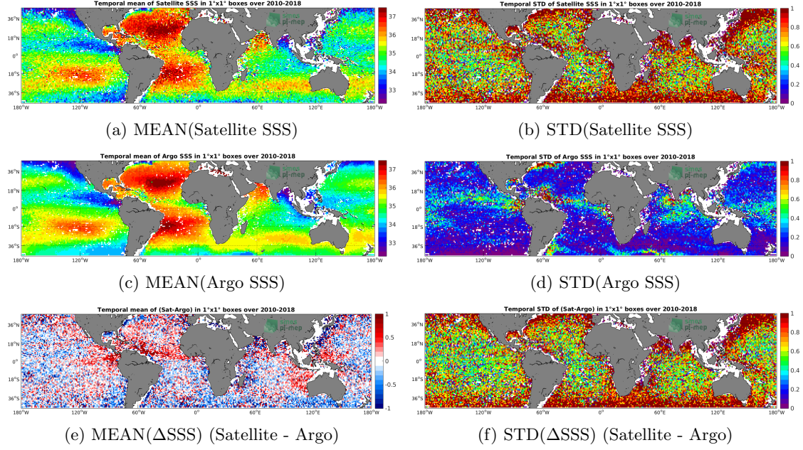
Figure 6: Temporal mean (left) and STD (right) of SSS from SMOS-L2-DPGS-v662 (top), Argo (middle), and of \Delta SSS (Satellite - Argo). Only match-up pairs are used to generate these maps.
