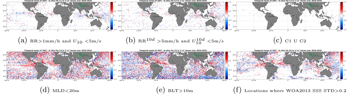
Figure 12: Temporal mean gridded over spatial boxes of size 1^\circ \times 1^\circ of \Delta\text{SSS} (SMOS-L2-DPGS-v662 - Argo) for 6 different subdatasets corresponding to: \text{RR} > 1\text{mm/h} and U_{10} < 5\text{m/s} (a), \text{RR}^{10d} > 5\text{mm/h} and U_{10}^{10d} < 5\text{m/s} (b), C1 U C2 (c), \text{MLD} < 20\text{m} (d), \text{BLT} > 10\text{m} (e), Locations where WOA2013 SSS STD > 0.2 (f).
