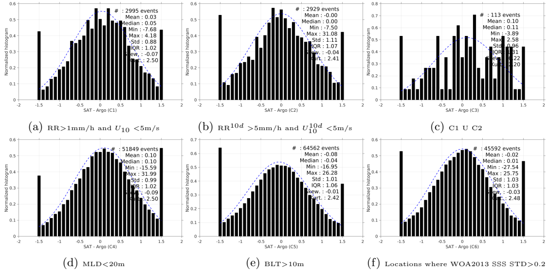
Figure 13: Normalized histogram of \Delta\text{SSS} (SMOS-L2-DPGS-v662 - Argo) for 6 different subdatasets corresponding to: \text{RR}>1\text{mm/h} and U_{10} <5\text{m/s} (a), \text{RR}^{10d} >5\text{mm/h} and U_{10}^{10d} <5\text{m/s} (b), C1 U C2 (c), \text{MLD}<20\text{m} (d), \text{BLT}>10\text{m} (e), Locations where WOA2013 SSS STD >0.2 (f).
