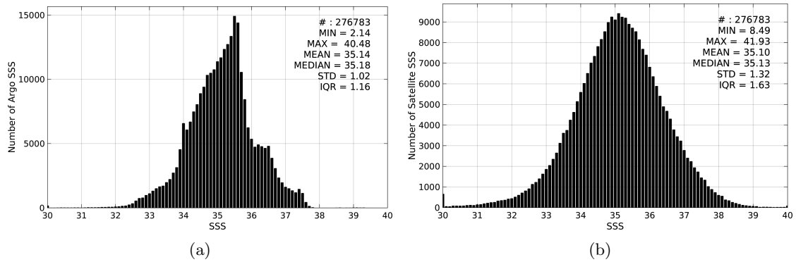
Figure 2: Histograms of SSS from Argo (a) and SMOS-L2-DPGS-v662 (b) considering all match-up pairs per bins of 0.1 over the Mid-Low Latitudes 45N-45S Pi-MEP region and for the full satellite product period.
