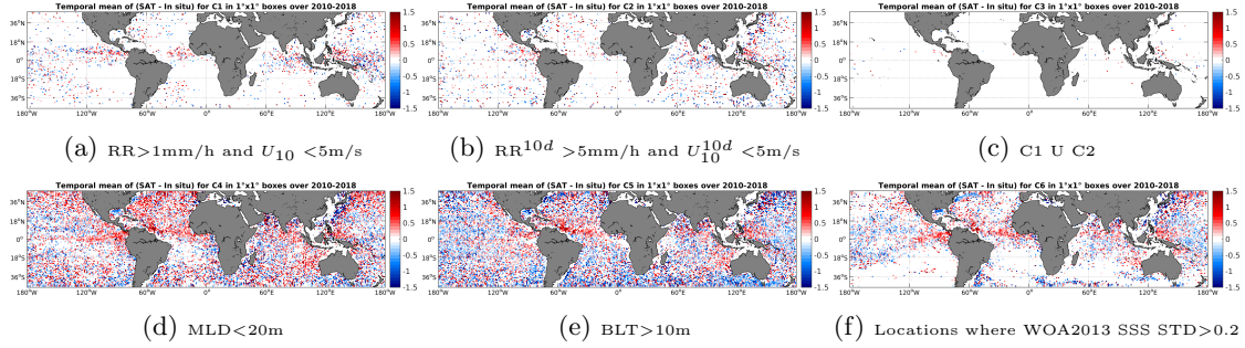
Figure 12: Temporal mean gridded over spatial boxes of size 1^\circ \times 1^\circ of \Delta\text{SSS} (SMOS-L2-DPGS-v662 - Argo) for 6 different subdatasets corresponding to: \text{RR}>1\text{mm/h} and U_{10} <5\text{m/s} (a), \text{RR}^{10d} >5\text{mm/h} and U_{10}^{10d} <5\text{m/s} (b), C1 U C2 (c), \text{MLD}<20\text{m} (d), \text{BLT}>10\text{m} (e), Locations where WOA2013 SSS STD >0.2 (f).
