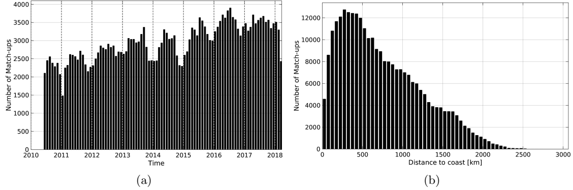
Figure 1: Number of match-ups between Argo and SMOS-L2-DPGS-v662 SSS as a function of time (a) and as function of the distance to coast (b) over the Mid-Low Latitudes 45N-45S Pi-MEP region and for the full satellite product period.
