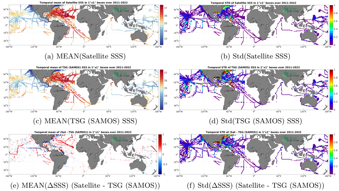
Figure 6: Temporal mean (left) and Std (right) of SSS from SMAP SSS L4 OI v1 - 7 Days (IPRC) (top), TSG (SAMOS) (middle), and of \Delta SSS (Satellite - TSG (SAMOS)). Only match-up pairs are used to generate these maps.
