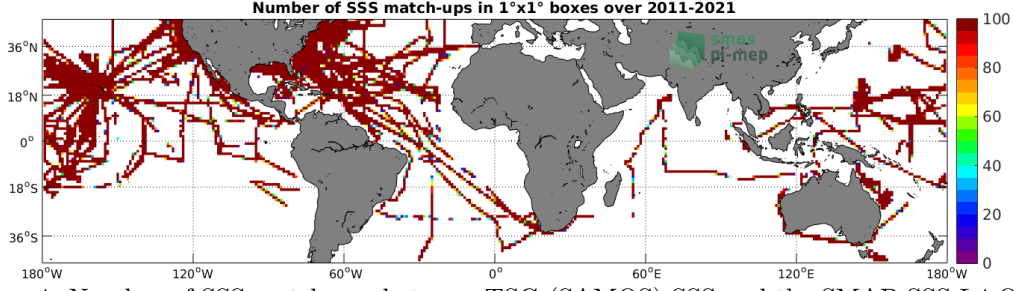
Figure 4: Number of SSS match-ups between TSG (SAMOS) SSS and the SMAP SSS L4 OI v1 - 7 Days (IPRC) SSS product for the Mid-Low Latitudes 45N-45S Pi-MEP region over 1^\circ \times 1^\circ boxes and for the full satellite product period.
