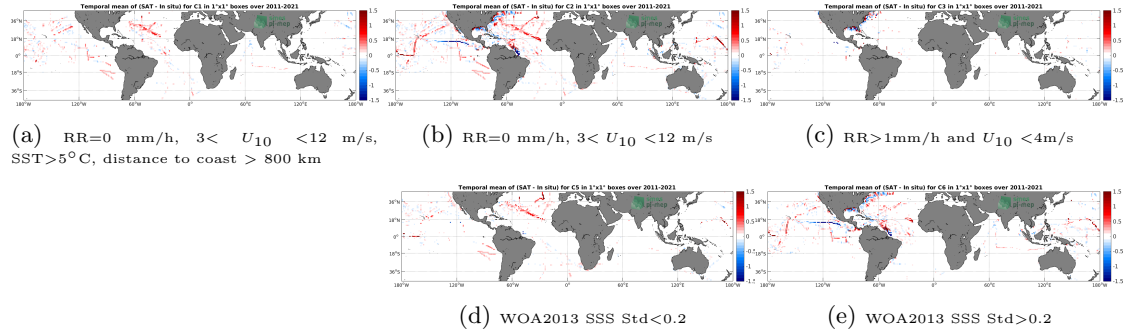
Figure 12: Temporal mean gridded over spatial boxes of size 1^\circ \times 1^\circ of \Delta SSS (SMAP SSS L4 OI v1 - 7 Days (IPRC) - TSG (SAMOS)) for 5 different subdatasets corresponding to:RR=0 mm/h, 3 < U_{10} < 12 m/s, SST >5^\circ\text{C} , distance to coast > 800 km (a), RR=0 mm/h, 3 < U_{10} < 12 m/s (b), RR >1 mm/h and U_{10} < 4 m/s (c), WOA2013 SSS Std <0.2 (d), WOA2013 SSS Std >0.2 (e).
