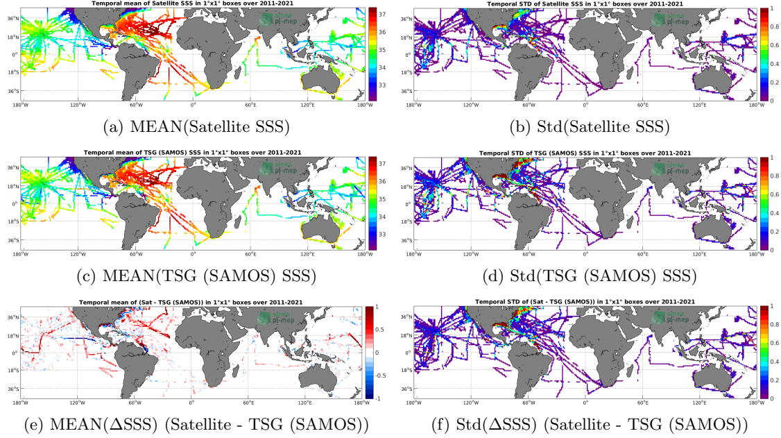
Figure 6: Temporal mean (left) and Std (right) of SSS from SMAP SSS L4 OI v1 - 7 Days (IPRC) (top), TSG (SAMOS) (middle), and of \Delta SSS (Satellite - TSG (SAMOS)). Only match-up pairs are used to generate these maps.
