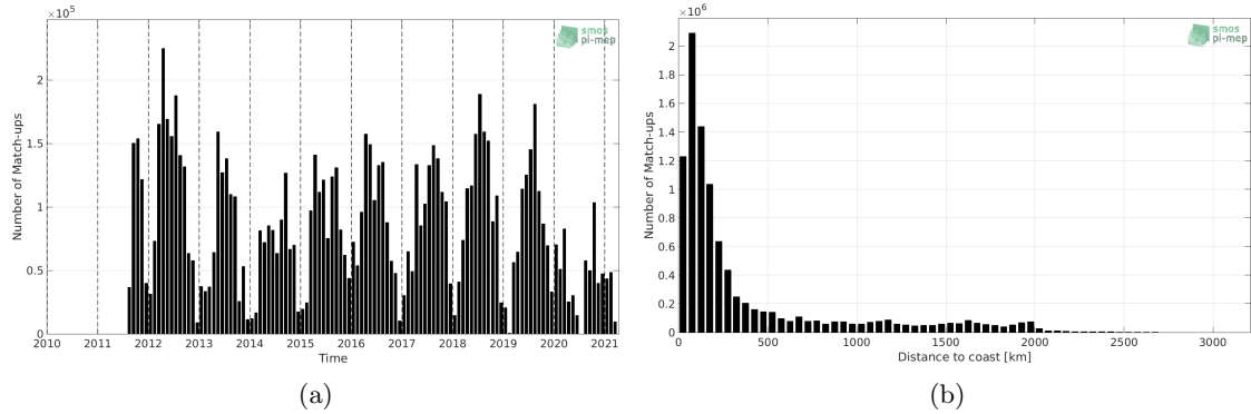
Figure 1: Number of match-ups between TSG (SAMOS) and SMAP SSS L4 OI v1 - 7 Days (IPRC) SSS as a function of time (a) and as function of the distance to coast (b) over the Mid-Low Latitudes 45N-45S Pi-MEP region and for the full satellite product period.
