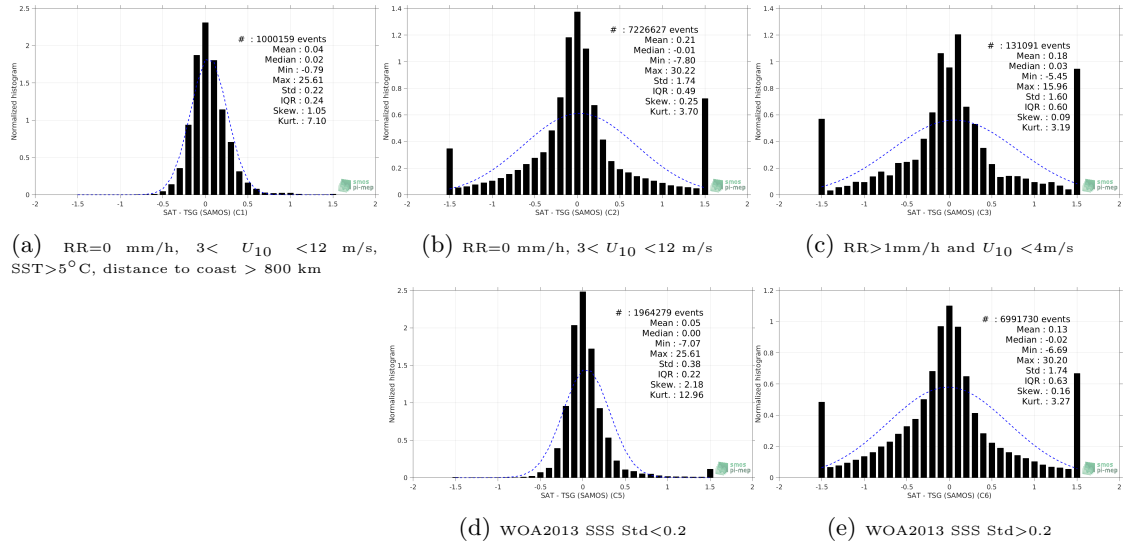
Figure 13: Normalized histogram of \Delta SSS (SMAP SSS L4 OI v1 - 7 Days (IPRC) - TSG (SAMOS)) for 5 different subdatasets corresponding to: RR=0 mm/h, 3 < U_{10} < 12 m/s, SST >5^\circ\text{C} , distance to coast > 800 km (a), RR=0 mm/h, 3 < U_{10} < 12 m/s (b), RR >1 mm/h and U_{10} < 4 m/s (c), WOA2013 SSS Std <0.2 (d), WOA2013 SSS Std >0.2 (e).
