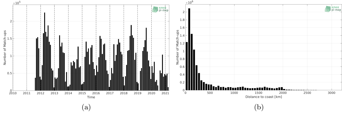
Figure 1: Number of match-ups between TSG (SAMOS) and SMAP SSS L4 OI v1 - 7day (IPRC) SSS as a function of time (a) and as function of the distance to coast (b) over the Mid-Low Latitudes 45N-45S Pi-MEP region and for the full satellite product period.
