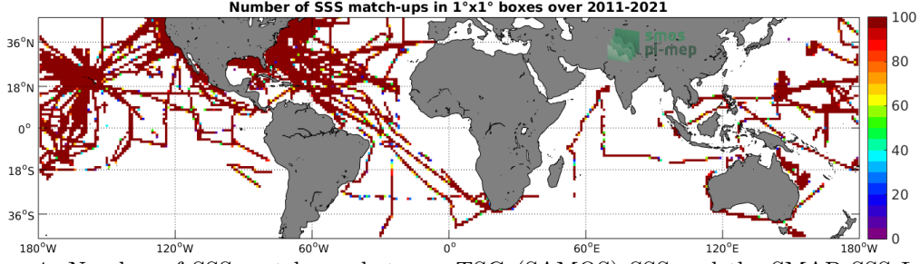
Figure 4: Number of SSS match-ups between TSG (SAMOS) SSS and the SMAP SSS L4 OI v1 - 7day (IPRC) SSS product for the Mid-Low Latitudes 45N-45S Pi-MEP region over 1^\circ \times 1^\circ boxes and for the full satellite product period.
