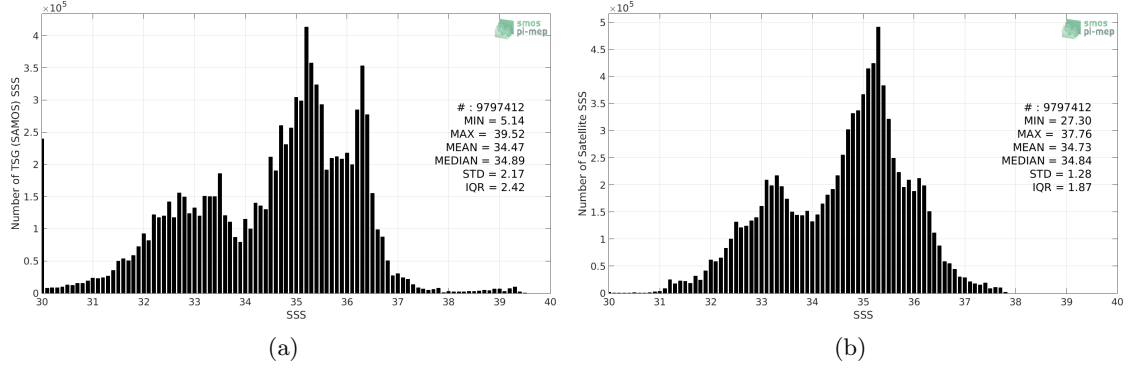
Figure 2: Histograms of SSS from TSG (SAMOS) (a) and SMAP SSS L4 OI v1 - 7day (IPRC) (b) considering all match-up pairs per bins of 0.1 over the Mid-Low Latitudes 45N-45S Pi-MEP region and for the full satellite product period.
