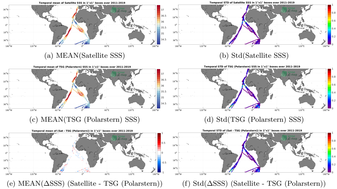
Figure 6: Temporal mean (left) and Std (right) of SSS from SMAP SSS L4 OI v1 - 7 Days (IPRC) (top), TSG (Polarstern) (middle), and of \Delta SSS (Satellite - TSG (Polarstern)). Only match-up pairs are used to generate these maps.
