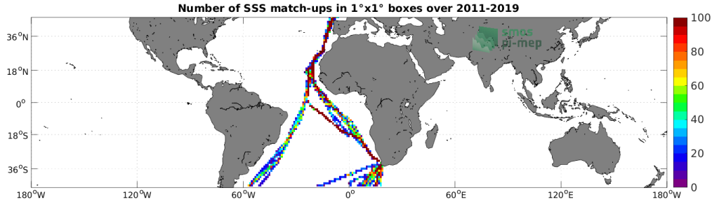
Figure 4: Number of SSS match-ups between TSG (Polarstern) SSS and the SMAP SSS L4 OI v1 - 7 Days (IPRC) SSS product for the Mid-Low Latitudes 45N-45S Pi-MEP region over 1^\circ \times 1^\circ boxes and for the full satellite product period.
