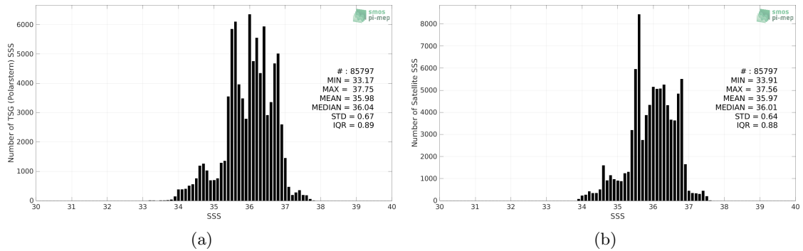
Figure 2: Histograms of SSS from TSG (Polarstern) (a) and SMAP SSS L4 OI v1 - 7 Days (IPRC) (b) considering all match-up pairs per bins of 0.1 over the Mid-Low Latitudes 45N-45S Pi-MEP region and for the full satellite product period.
