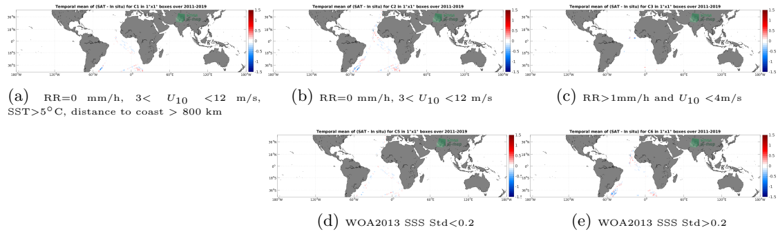
Figure 12: Temporal mean gridded over spatial boxes of size 1^\circ \times 1^\circ of \Delta SSS (SMAP SSS L4 OI v1 - 7 Days (IPRC) - TSG (Polarstern)) for 5 different subdatasets corresponding to:RR=0 mm/h, 3 < U_{10} < 12 m/s, SST >5^\circ C, distance to coast > 800 km (a), RR=0 mm/h, 3 < U_{10} < 12 m/s (b), RR >1 mm/h and U_{10} < 4 m/s (c), WOA2013 SSS Std <0.2 (d), WOA2013 SSS Std >0.2 (e).
