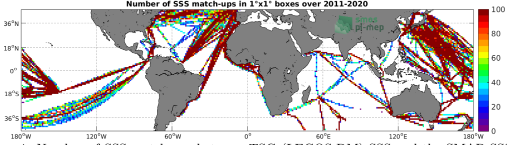
Figure 4: Number of SSS match-ups between TSG (LEGOS-DM) SSS and the SMAP SSS L4 OI v1 - 7 Days (IPRC) SSS product for the Mid-Low Latitudes 45N-45S Pi-MEP region over 1^\circ \times 1^\circ boxes and for the full satellite product period.
