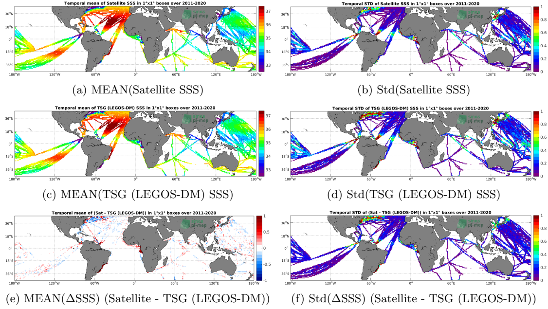
Figure 6: Temporal mean (left) and Std (right) of SSS from SMAP SSS L4 OI v1 - 7 Days (IPRC) (top), TSG (LEGOS-DM) (middle), and of \Delta SSS (Satellite - TSG (LEGOS-DM)). Only match-up pairs are used to generate these maps.
