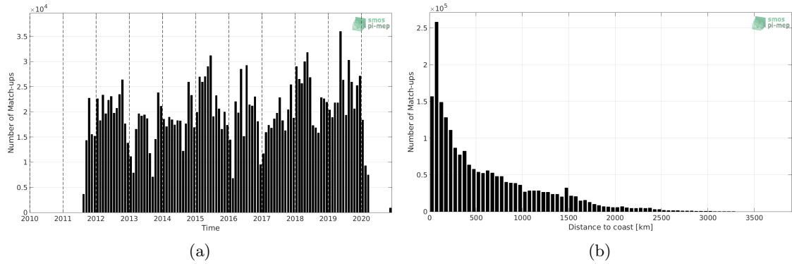
Figure 1: Number of match-ups between TSG (LEGOS-DM) and SMAP SSS L4 OI v1 - 7 Days (IPRC) SSS as a function of time (a) and as function of the distance to coast (b) over the Mid-Low Latitudes 45N-45S Pi-MEP region and for the full satellite product period.
