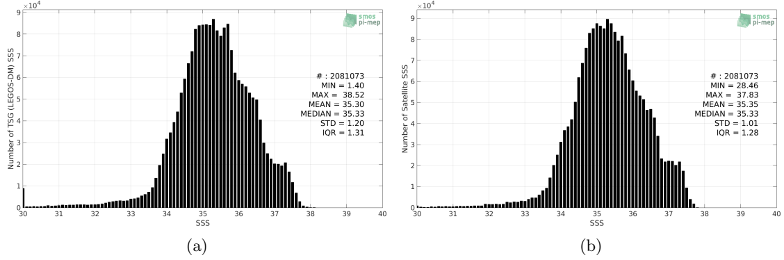
Figure 2: Histograms of SSS from TSG (LEGOS-DM) (a) and SMAP SSS L4 OI v1 - 7 Days (IPRC) (b) considering all match-up pairs per bins of 0.1 over the Mid-Low Latitudes 45N-45S Pi-MEP region and for the full satellite product period.
