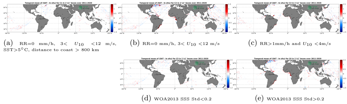
Figure 12: Temporal mean gridded over spatial boxes of size 1^\circ \times 1^\circ of \Delta SSS (SMAP SSS L4 OI v1 - 7day (IPRC) - TSG (LEGOS-DM)) for 5 different subdatasets corresponding to: RR=0 mm/h, 3 < U_{10} < 12 m/s, SST > 5^\circ C , distance to coast > 800 km (a), RR=0 mm/h, 3 < U_{10} < 12 m/s (b), RR > 1 mm/h and U_{10} < 4 m/s (c), WOA2013 SSS Std < 0.2 (d), WOA2013 SSS Std > 0.2 (e).
