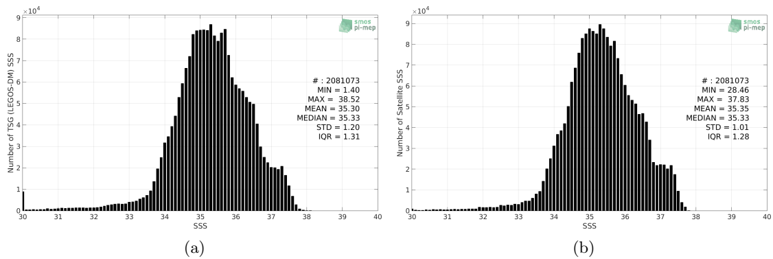
Figure 2: Histograms of SSS from TSG (LEGOS-DM) (a) and SMAP SSS L4 OI v1 - 7day (IPRC) (b) considering all match-up pairs per bins of 0.1 over the Mid-Low Latitudes 45N-45S Pi-MEP region and for the full satellite product period.
