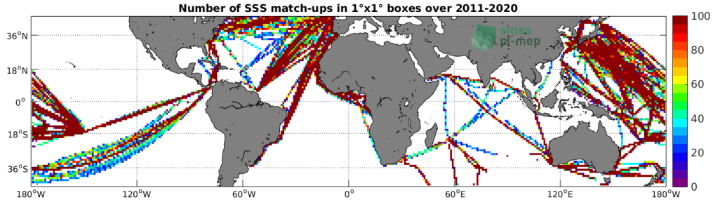
Figure 4: Number of SSS match-ups between TSG (LEGOS-DM) SSS and the SMAP SSS L4 OI v1 - 7day (IPRC) SSS product for the Mid-Low Latitudes 45N-45S Pi-MEP region over 1^\circ \times 1^\circ boxes and for the full satellite product period.
