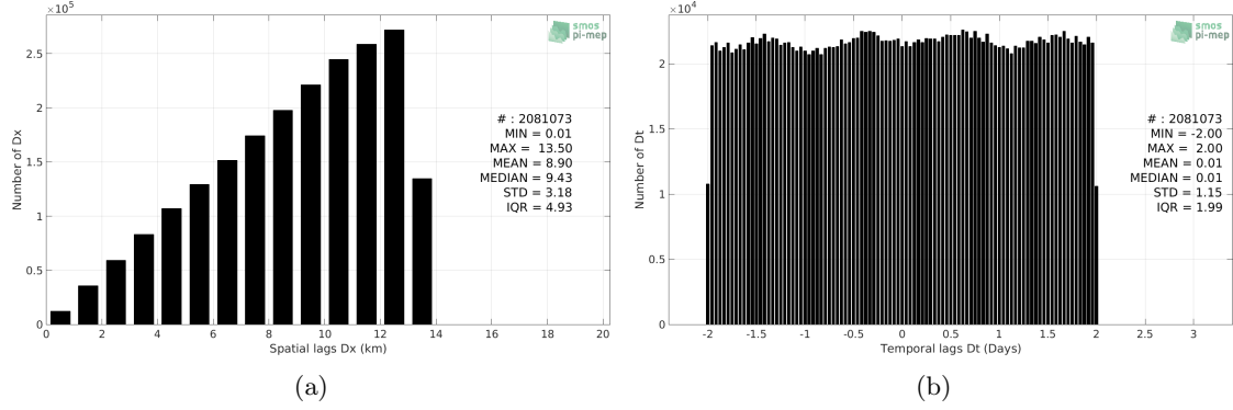
Figure 5: Histograms of the spatial (a) and temporal (b) lags between the location/time of the TSG (LEGOS-DM) measurement and the date of the corresponding SMAP SSS L4 OI v1 - 7day (IPRC) SSS pixel.
